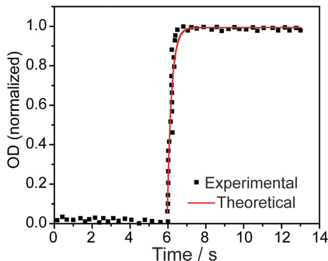
Figure 5. Local kinetics of the nucleation regime ahead the interface. Time-dependence of the normalized local optical density (OD) upon heating along a line perpendicular to the front propagation direction. The red curve is the best fit obtained using equation 2.
