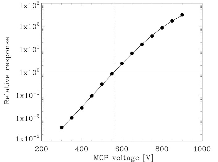
Fig. 21. Relative response of the HRI Lya camera vs. voltage applied to the MCP of the intensifier normalised at 560 V.
