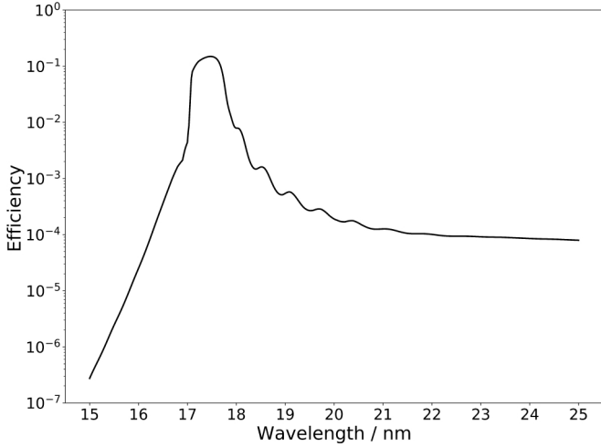
Fig. 22. Expected spectral response of \text{HRI}_{\text{EUV}} , assuming rear filter in open position. A detailed description can be found in Gissot & EUI consortium partners (in prep.).
