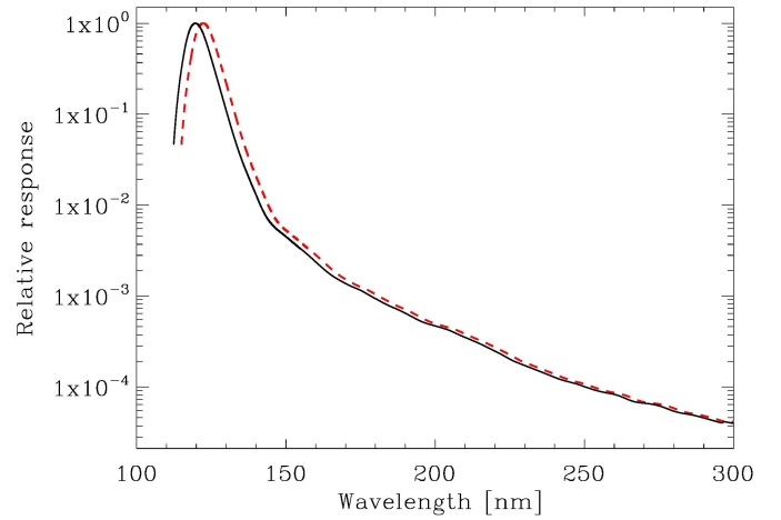
Fig. 24. Relative spectral response of \text{HRI}_{\text{Lya}} as predicted by the measured (black solid) and the theoretical efficiencies of the components (red dashed). A detailed description can be found in Schühle & EUI consortium partners (in prep.).
