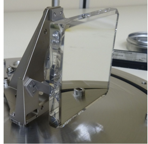
Fig. 8. FSI mirror coated and bonded on its mount.
