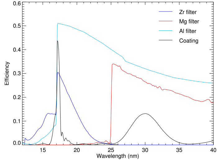
Fig. 6. Spectral selection in FSI. The multi-layer coating (black curve) reflects two bands centred at 17.4 nm and 30.4 nm. Zirconium (blue curve) and magnesium (red curve) filters are inserted in the beam near the focal plane to select one or the other. The entrance aluminium filter (light blue curve) transmits both bands. Data are from samples of the flight items.
