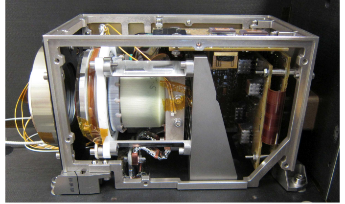
Fig. 15. HRI Lya camera with the APS sensor mounted in the middle, the Front End Electronics (FEE) on the right hand side, and the intensifier on the left hand side. See also Fig. 16 for a schematic layout.
