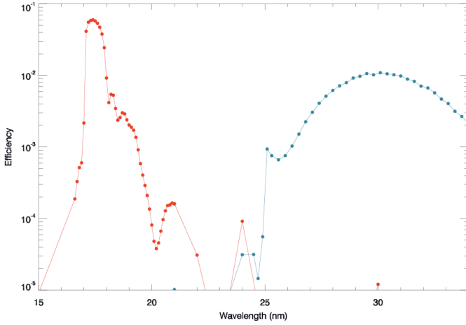
Fig. 23. Relative spectral response of the EUI/FSI channel from 15 to 34 nm, showing the 17.4 nm channel in red and the 30.4 nm channel in blue. A detailed description can be found in Auchère & EUI consortium partners (in prep.).
