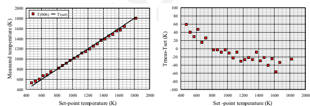
(b) evolution of the temperature determined with respect to the position of the sapphire 0,0,6 RLN as a function of the set-point temperature and evolution of discrepancy between the measured and set-point temperatures.
