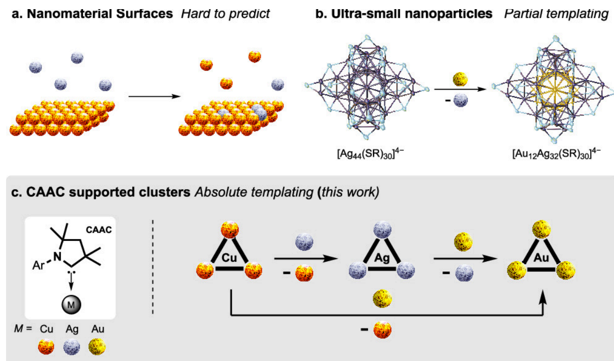
Figure 1. (a) Galvanic exchange on a metal surface involving the replacement of a more active metal (orange atom) for a less reducing one (gray atom) is hard to predict. (b) A rare example of multiple atom galvanic exchange in nanoclusters without loss of structural integrity.(11) (c) The stabilization provided by cyclic(alkyl)(amino)carbenes (CAACs) allows for the absolute templating of trinuclear clusters by galvanic exchange.
