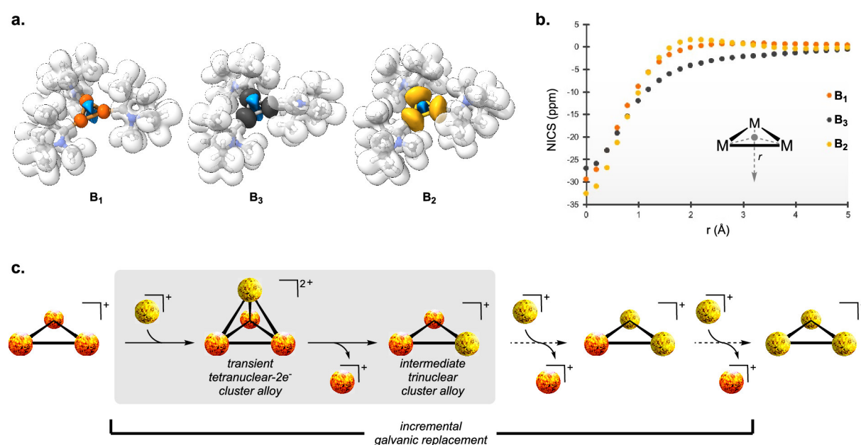
Figure 3. (a) Electron localization function (ELF) in B 1 – B 3 highlights a trisynaptic basin (blue) of a three-center two-electron cycle. (b) The \sigma -aromaticity in trinuclear B 1 – B 3 is indicated by the NICS scan plots showing large negative values at the ring center, gradually increasing to zero moving away from the ring center. (21) (c) The galvanic templating is proposed to involve sequential and incremental galvanic replacement via transient tetranuclear 4-center-2e – clusters.
