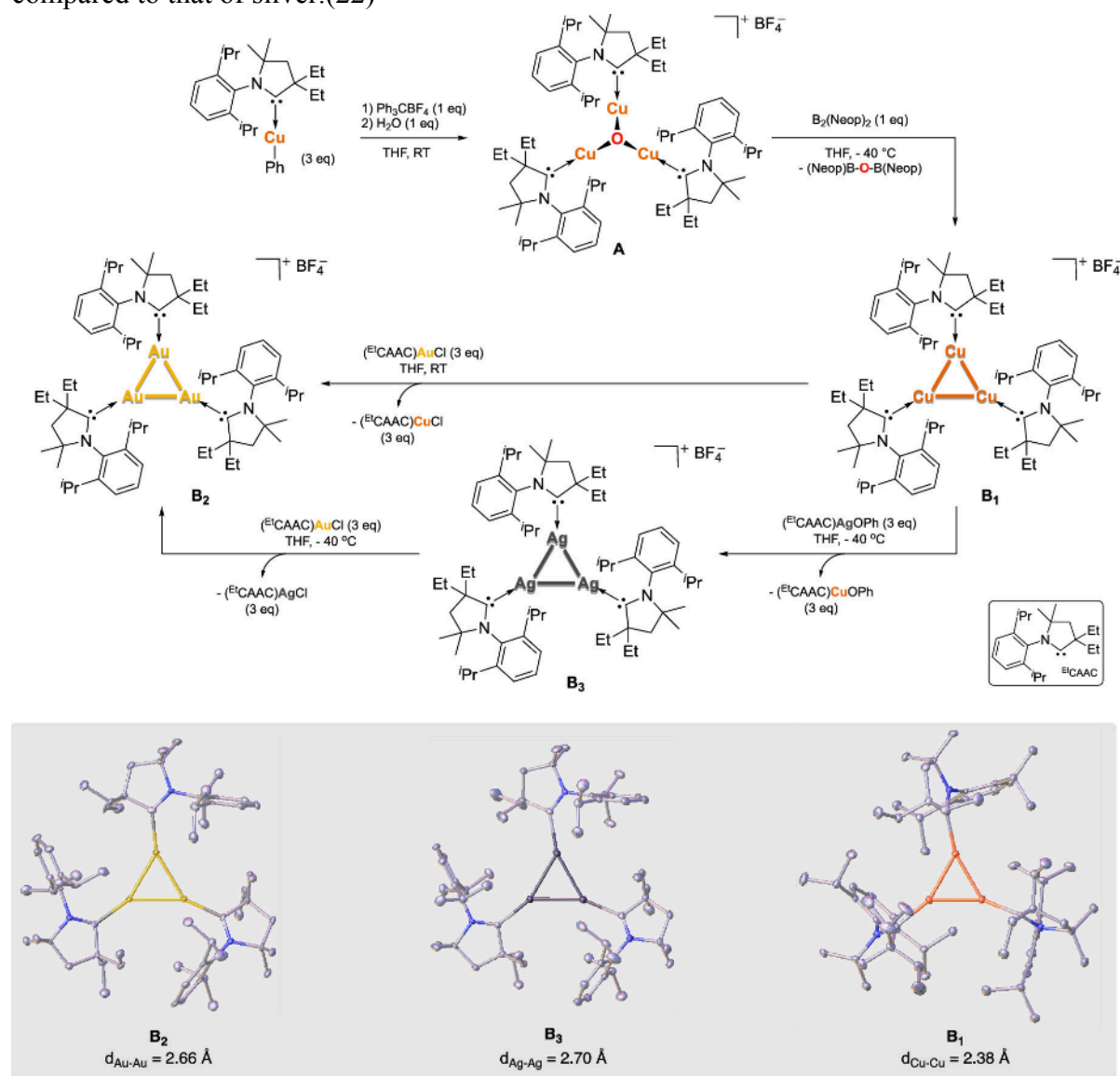
Figure 2. (Top) Trinuclear Cu 0 2 Cu 1 B 1 obtained by reduction of the μ 3 -oxo-[Cu( Et CAAC)] 3 A , allows for the absolute templating of trinuclear M 0 2 M 1 by galvanic exchange across the entire coinage metal series without loss of structural integrity. (Bottom) X-ray structures of trinuclear B 1 – B 3 ; anions and hydrogens have been omitted for clarity.
