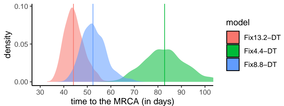
Figure 2. Time to the origin of the French epidemic wave as a function of the molecular clock. This estimate was obtained assuming an exponential growth coalescent population model and a fixed molecular clock (see Figure S4 for the BDSKY model). Colors indicate substitution rates and numbers (4.4, 8.8, 13.4) refer values to be multiplied by 10^{-4} substitutions/site/year. The slower the clock rate, the further away in time the most recent common ancestor (MRCA). Vertical lines show the distribution medians. The most recent sample dates from Mar 24, 2020.
