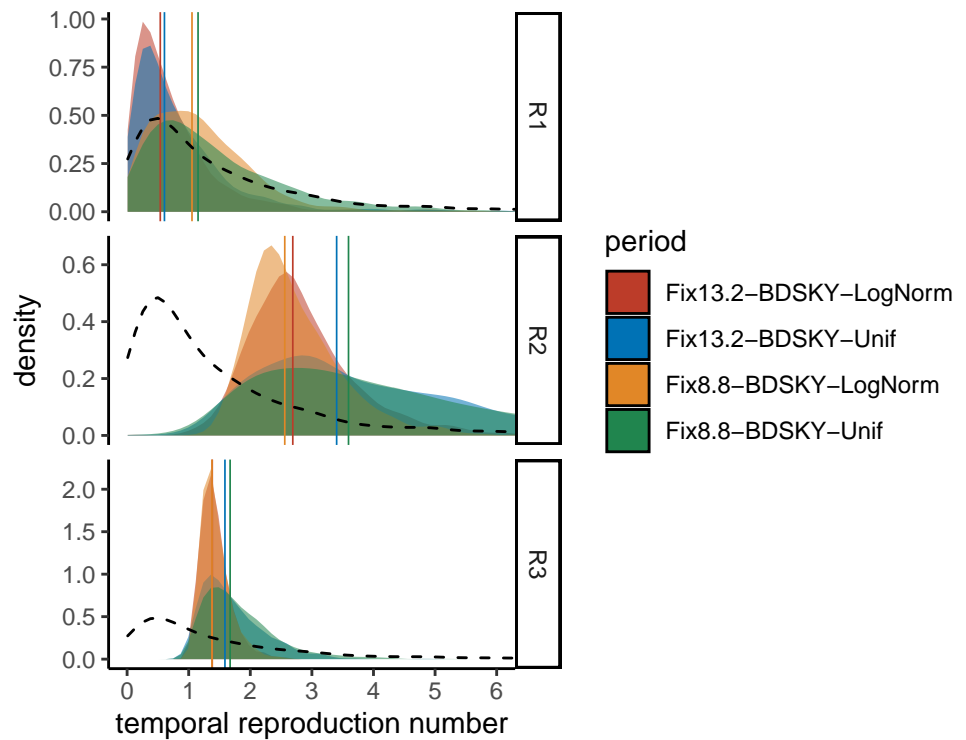
Figure S9. Effect of the prior shape and of the molecular clock on the temporal reproduction number estimate. The molecular clock value has a stronger effect than the prior shape except for \mathcal{R}_3 , where the effect is limited. For \mathcal{R}_1 , posterior distributions are close to the prior (black dashed line), as discussed in the main text.
