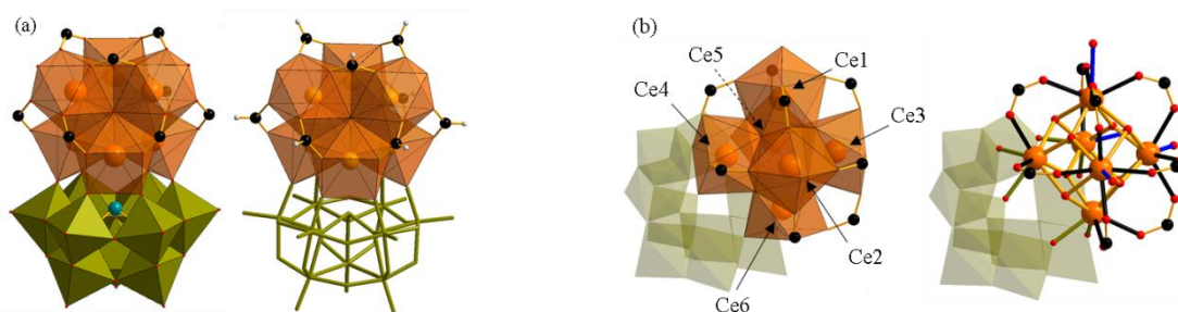
Figure 2: (a) Structural representation of compound 2 and (b) highlight and labels of the cerium cluster. \{WO_6\} : green polyhedron, \{CeO_n, n=8-9\} : orange polyhedron, C: black spheres, Na: blue spheres and H: white spheres. Ce-O bonds with the polyanion are in green, with the formate ligands in black, with the central oxo/hydroxo bridges in orange and with water in blue.
