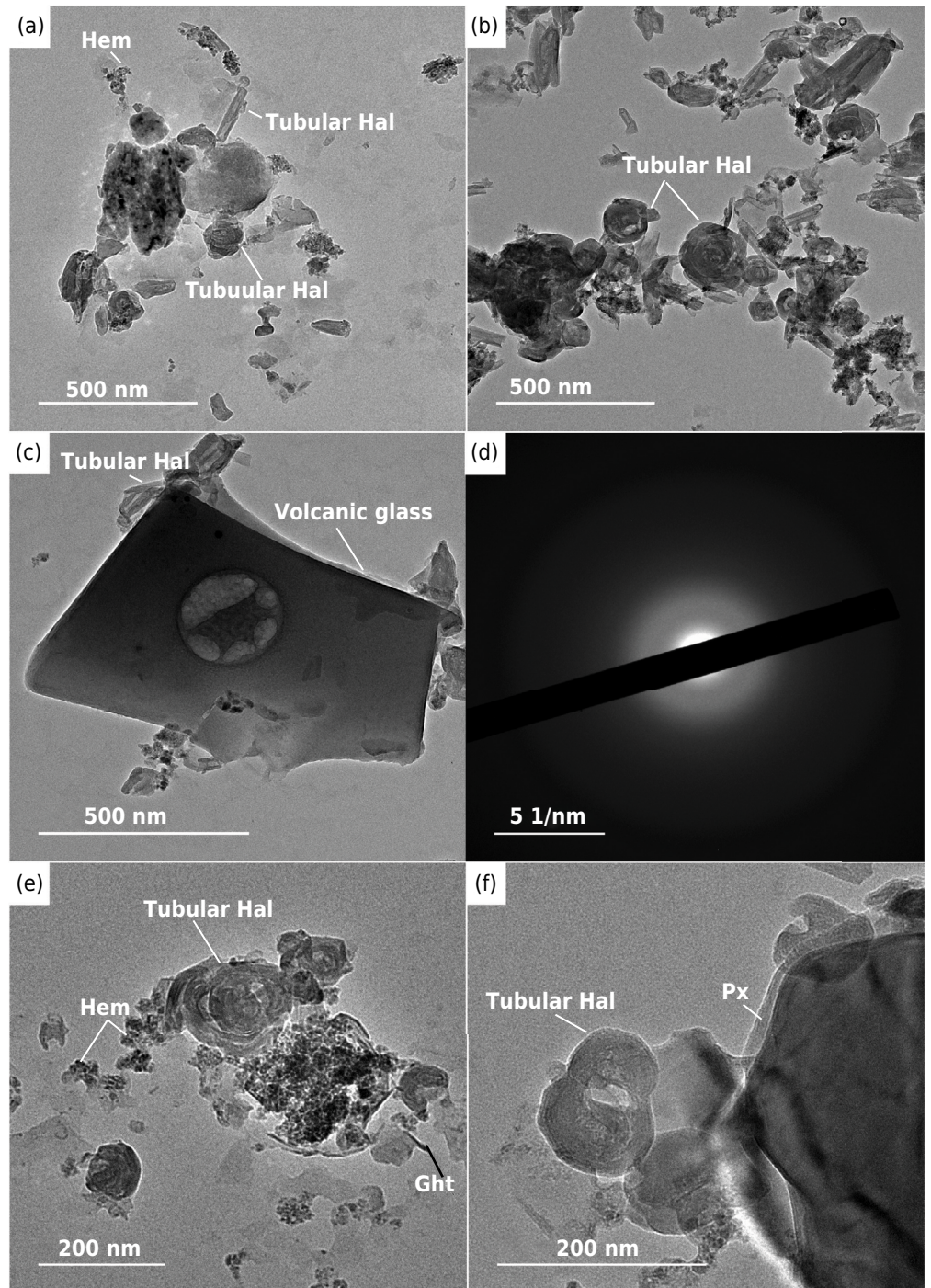
Figure 7. Transmission Electron Microscope images of fraction clay of P1. Tubular halloysite and iron oxides (hematite) in pyroclast (a). Tubular halloysite in C2 horizon (b). It is noted that the halloysite are very crystallized. Volcanic glass and halloysite in C2 horizon (c). Microdiffraction with a characteristic of amorphous material (d). Tubular halloysite iron oxyhydroxides (globular hematite and acicular goethite) in Bi horizon (e). Tubular halloysite near to the crystal pyroxene in A horizon (f). Hal: halloysite; Hem: hematite; Ght: goethite; Px: pyroxene.
