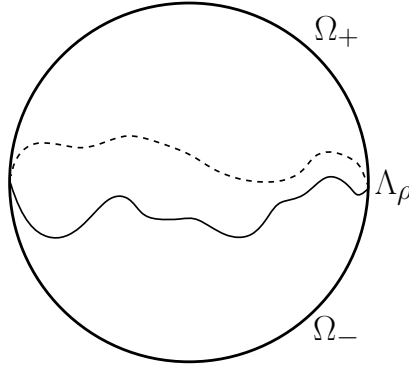
FIGURE 7. A picture of the limit set \widetilde{\Lambda}_\rho , which is a topological (n-1) -sphere and disconnects \partial\mathbb{H}^{n+1} in two connected components \Omega_+ and \Omega_- , which are homeomorphic to n -discs.
