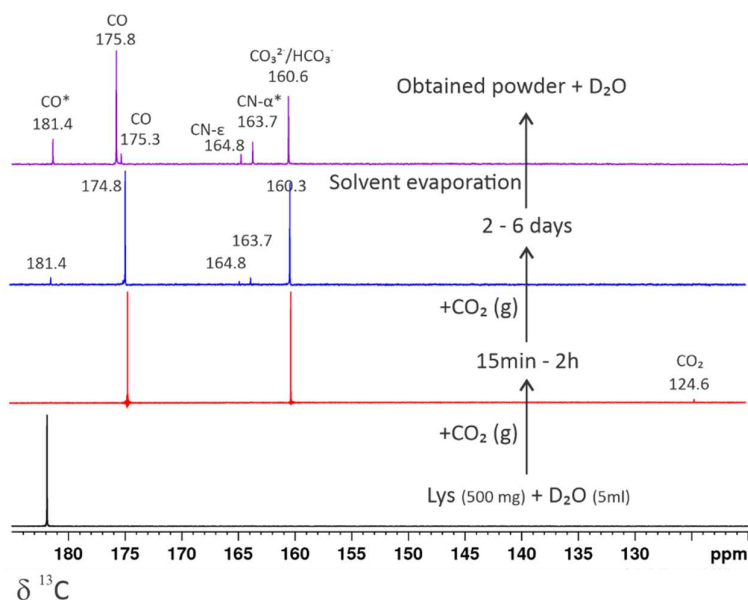
Figure 3: The ^{13}\text{C} NMR spectra of L-lysine solubilized in D 2 O (black spectrum), bubbling \text{CO}_2 (g) into the aqueous L-lysine for 15 min to 2h (red spectrum), bubbling \text{CO}_2 (g) into the aqueous solution for 2-6 days (blue spectrum), and after the solvent evaporation (purple spectrum).
