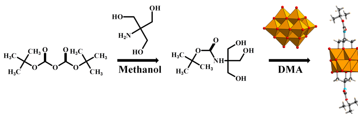
Figure 1. Synthetic pathway leading to the [V_6O_{13}\{(OCH_2)_3C-NH(BOC)\}_2]^{2-} anion.
