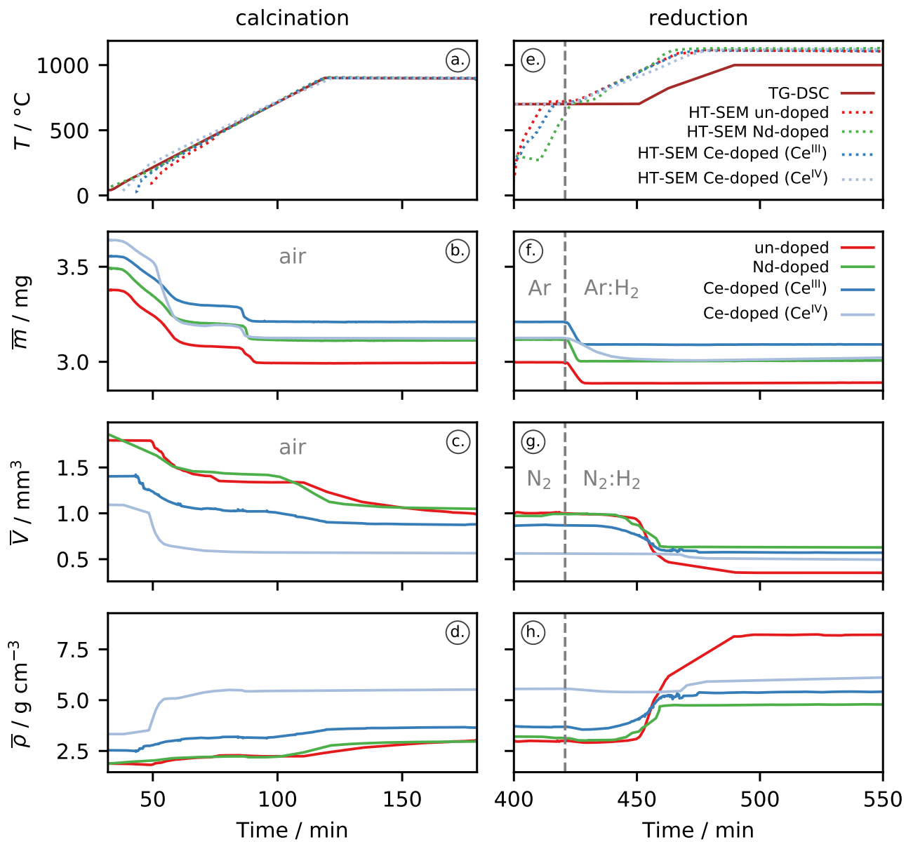
Figure 10: Temperatures measured during the TG-DSC and HT-SEM analyses for the calcination in air (a) and sintering in reducing atmosphere (e). Masses obtained during the TG-DSC measurements standardised to the average particle masses (b, f) and volumes derived from radii measured in the HT-SEM investigations standardised to the average particle volumes (c, g), as well as resulting average in-situ particle densities during both thermal treatment steps (d, h).
