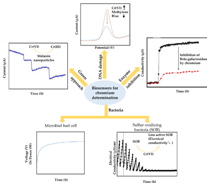
Figure 4. Scheme of different used biosensors for chromium determination.
