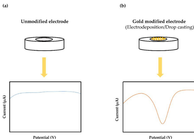
Figure 3. Typical response of Cr(VI) at: (a) unmodified; (b) AuNPs modified electrode using electrodeposition or drop casting strategy.
