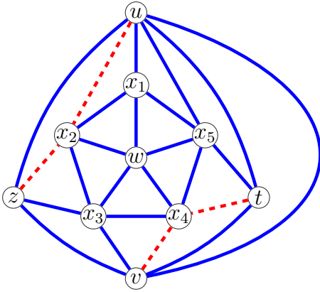
Figure 6: Signed graph H_1
