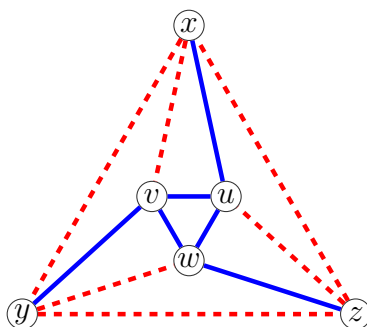
Figure 2: (2, 0) -coloring a negative triangle
