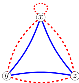
Figure 11: T^- does not bound \mathcal{SP}
