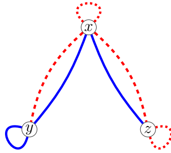
Figure 16: T_2 does not bound \mathcal{SP} ?
