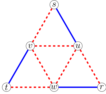
Figure 13: (G, \sigma) \not\rightarrow T' - z
