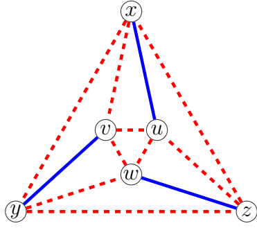
Figure 3: (1, 1) -coloring a negative triangle Figure 4: (1, 1) -coloring a positive triangle
