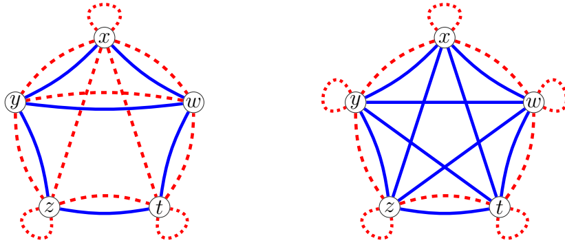
Figure 19: 5-vertices bound on \mathcal{SP} ?
