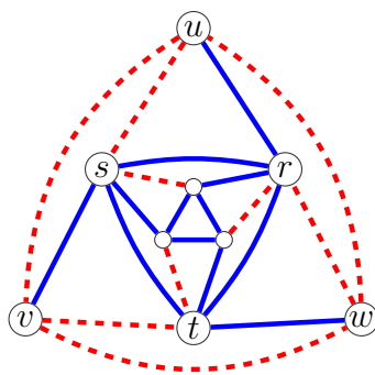
Figure 17: T_2 -coloring a negative triangle
