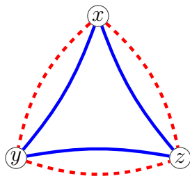
Figure 8: Smallest not (2, 0) -colorable graph without a loop
