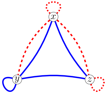
Figure 15: Does T_1 bound \mathcal{SP} ?
