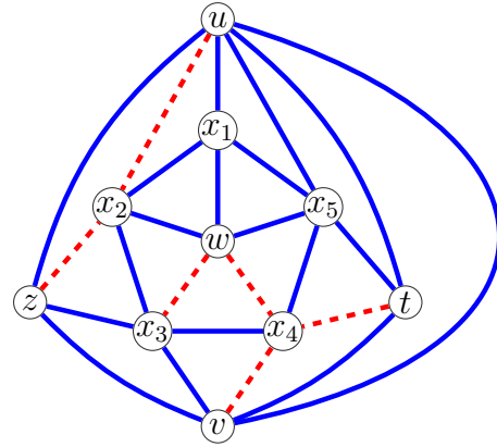
Figure 7: Signed graph H_2
