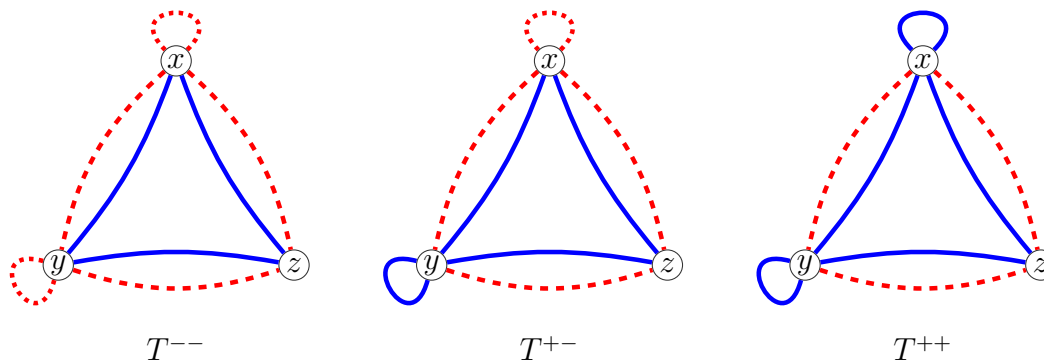
Figure 10: Three minimal homomorphism bounds of signed planar simple graphs
