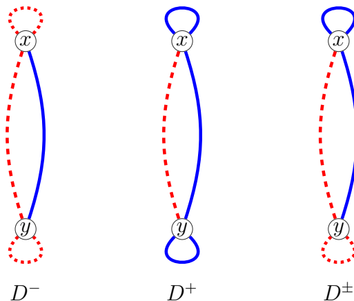
Figure 1: The homomorphism targets for complex 4-coloring
