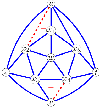
Figure 5: Gadget to forbid opposite colors on two vertices
