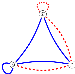
Figure 12: T^{+-} - (xy)^- does not bound \mathcal{SP}
