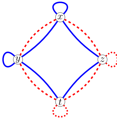
Figure 18: The configuration associated to Problem 20
