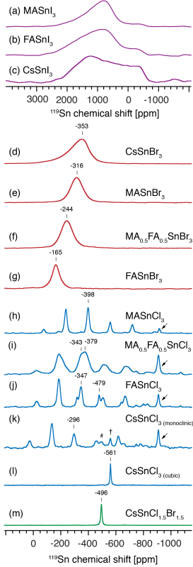
Figure 4. ^{119}\text{Sn} as a probe of the A-site cation (Cs, MA, FA) and A-site cation mixing in tin(II) halide perovskites. ^{119}\text{Sn} solid-state MAS NMR spectra at 4.7 T, 12 kHz MAS (unless stated otherwise) and 298 K of iodides: (a) \text{MASnI}_3 , (b) \text{FASnI}_3 (static, see fig. S6 for 12 kHz MAS) (c) \text{CsSnI}_3 ; bromides: (d) \text{CsSnBr}_3 , (e) \text{MASnBr}_3 , (f) \text{MA}_{0.5}\text{FA}_{0.5}\text{SnBr}_3 , (g) \text{FASnBr}_3 ; chlorides: (h) \text{MASnCl}_3 , (i) \text{MA}_{0.5}\text{FA}_{0.5}\text{SnCl}_3 , (j) \text{FASnCl}_3 , (k) \text{CsSnCl}_3 (monoclinic), † indicates the metastable cubic phase of \text{CsPbI}_3 , # is likely a second tin(II) site in the asymmetric unit cell of \text{CsPbCl}_3 (l) \text{CsSnCl}_3 (cubic); mixed-halides: (m) \text{CsSnCl}_{1.5}\text{Br}_{1.5} . The arrows indicate trace unreacted \text{SnCl}_2 .
