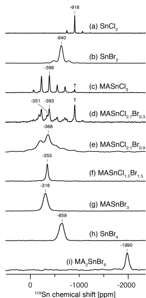
Figure 2. 119 Sn solid-state MAS NMR spectra of mixed-anion (chloride/bromide) halostannates and their precursors at 4.7 T, 12 kHz MAS (except for SnBr 4 ) and 298 K: (a) SnCl 2 , (b) SnBr 2 , (c) MASnCl 3 , (d) MASnCl 2.7 Br 0.3 , (e) MASnCl 2.1 Br 0.9 , (f) MASnCl 1.5 Br 1.5 , (g) MASnBr 3 , (h) SnBr 4 (at 0.6 kHz MAS to prevent melting), (i) MA 2 SnBr 6 , † indicates trace unreacted SnCl 2 .
