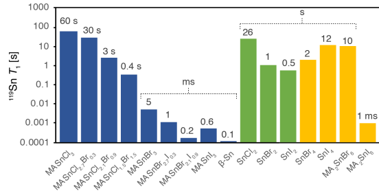
Figure 6. ^{119}\text{Sn} longitudinal relaxation times ( T_1 ) at 4.7 T, 298 K, 12 kHz MAS (except for \text{SnBr}_4 which was measured at 0.6 kHz MAS to prevent melting) of the tin(II)- and tin(IV)-containing phases investigated in this work. Blue: tin(II) halide perovskites, green: tin(II) halides, yellow: tin(IV) halides and halostannates(IV). The numerical values are reported in table S3
