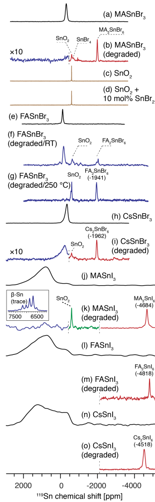
Figure 5. ^{119}\text{Sn} as a probe of tin(II) halide perovskite degradation. ^{119}\text{Sn} solid-state MAS NMR spectra at 4.7 T, 12 kHz MAS and 298 K of (a) \text{MASnBr}_3 (as prepared), (b) \text{MASnBr}_3 (degraded for 1 h at 250 °C in air), (c) \text{SnO}_2 , (d) \text{SnO}_2 + 10 \text{ mol}\% \text{SnBr}_2 (ground and annealed at 250 °C in air), (e) \text{FASnBr}_3 (as prepared), (f) \text{FASnBr}_3 (degraded for 5 days at RT, in air), (g) \text{FASnBr}_3 (degraded for 0.5 h at 250 °C in air), (h) \text{CsSnBr}_3 (as prepared), (i) \text{CsSnBr}_3 (degraded for 0.5 h at 350 °C in air), (j) \text{MASnI}_3 (as prepared), (k) \text{MASnI}_3 (degraded for 1 h at 150 °C in air), (l) \text{FASnI}_3 (as prepared), (m) \text{FASnI}_3 (degraded for 1 h at RT in air), (n) \text{CsSnI}_3 (as prepared), (o) \text{CsSnI}_3 (degraded for 3 h at 100 °C in air). The dashed lines indicate points at which spectra acquired at different transmitter offsets were stitched together: b, i (two offsets), k (three offsets). For m and o only the high-field (low ppm) part was acquired.
