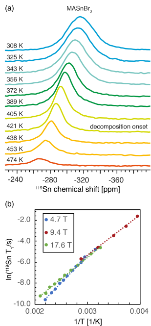
Figure 7. Halide dynamics in \text{MASnBr}_3 from multi-field variable-temperature ^{119}\text{Sn} solid-state MAS NMR. (a) variable-temperature (308–474 K) ^{119}\text{Sn} spectra at 17.6 T. All spectra were acquired using the same number of scans (4096) and are quantitative. The spectrum after thermal decomposition corresponds to \text{MA}_2\text{SnBr}_6 (fig. 4b) with traces of \text{SnO}_2 as discussed above. (b) An Arrhenius plot of the ^{119}\text{Sn} T_1 relaxation data at 4.7 T (blue), 9.4 T (red) and 17.6 T (green). The linear fits are indicated by dotted lines and the numerical values are given in table S2.
