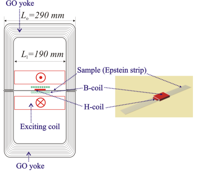
Fig. 1. The single-strip permeameter (adapted from [13]). The Epstein strip sample is endowed with a centrally located H -coil, enwrapped by a secondary B -coil.
