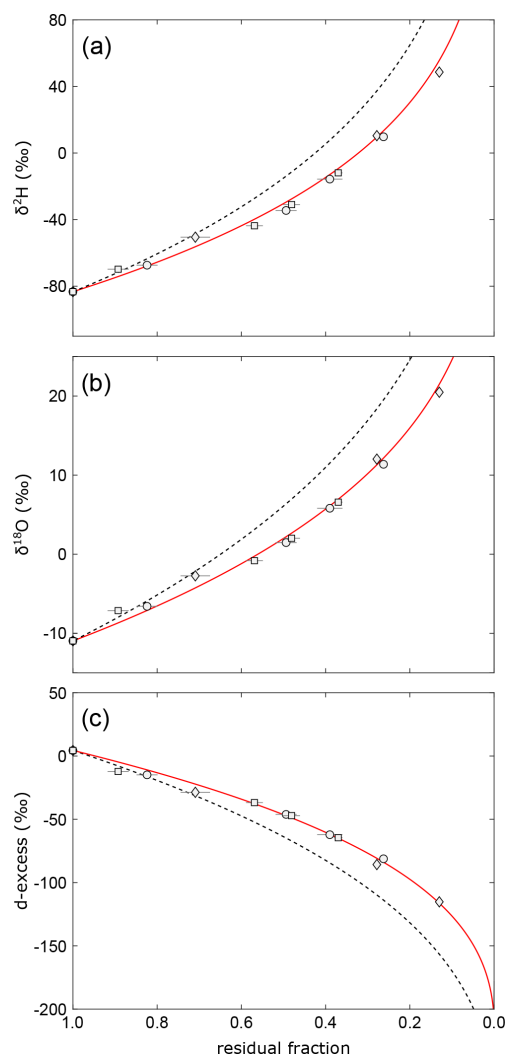
Figure 9. Isotopic evolution of remaining water in evaporation experiments, similar to Fig. 8. Here, the red lines show evaporation trajectories obtained by fitting the virtual outlet model ( n = 0.59 , outlet = 20 %). The dashed lines represent evaporation trajectories for the simple evaporation model obtained using the same turbulence coefficient as for the virtual outlet model.
