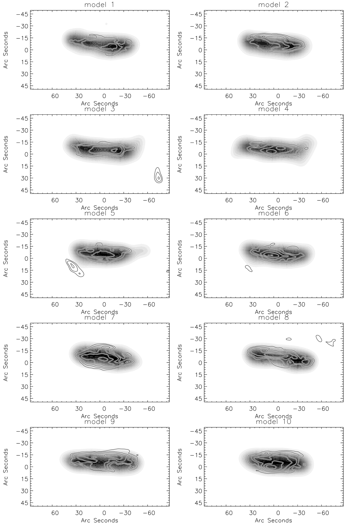
Fig. 13. Model polarized emission distributions on model H I distribution with i = 75^\circ .
