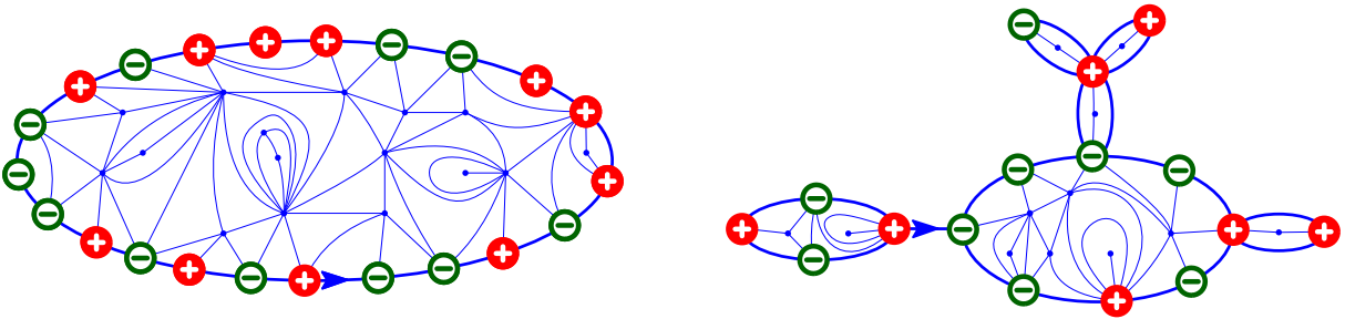
Figure 1: Two triangulations with boundary condition \omega = \ominus \ominus \ominus \ominus \ominus \ominus \oplus \oplus \oplus \oplus \oplus \oplus \oplus \oplus \oplus \oplus \ominus \ominus \ominus \ominus . The one on the left has a simple boundary whereas the one on the right has not.
