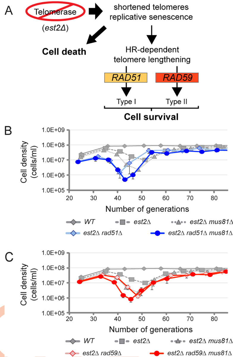
Fig 3. Reduced viability in the absence of MUS81 is independent of Type I or Type II telomerase-deficient survivor formation. (A) Diagram of survivor formation in the absence of yeast telomerase. Genetic requirements are highlighted for RAD51 and RAD59 in Type I and Type II survivor formation, respectively. Arrow size represents abundance of cells entering cell death or survival via homologous recombination (HR)-mediated telomere lengthening. (B) Average cell densities are plotted with one standard of error for wild type (WT) (n = 20), est2Δ (n = 40), est2Δ mus81Δ (n = 27), and est2Δ rad51Δ (n = 8), and est2Δ rad51Δ mus81Δ (n = 10), or (C) est2Δ rad59Δ (n = 9) and est2Δ rad59Δ mus81Δ (n = 9). Yeast strains rad51Δ , mus81Δ rad51Δ , est2Δ rad51Δ , and est2Δ rad51Δ mus81Δ strains were derived from diploid WDHY3358 as described in Materials and Methods. Remaining haploid strains, est2Δ rad59Δ , and est2Δ rad59Δ mus81Δ , were derived from WDHY3366, and est2Δ mus81- dd was derived from WDHY3007. WT and est2Δ strains were derived from sporulation of all three diploids.
