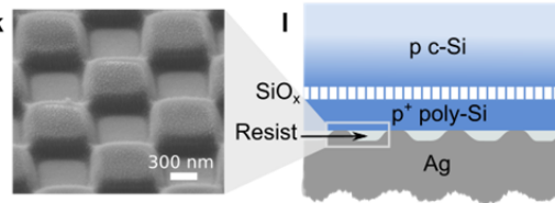
Figure 6. Techniques to fabricate nanostructures and examples of integration in solar cells. (a-f) Nanosphere lithography: (a) schematics of air-water colloidal assembly; (b) SEM image of a close-packed assembly of 700 nm-large polystyrene nanospheres 99 ; (c) schematics of a silicon solar cell integrating silica nanospheres at the rear 98 ; (d) schematics of sparse colloidal assembly relying on electrostatic interactions between charged colloids deposited on a oppositely charged substrate; (e) SEM image of the resulting amorphous colloidal distribution (sphere size: 270 nm) 101 ; (f) SEM side view of an ultrathin (1.1 μm) silicon solar cell nanotextured using sparse colloidal assembly 23 . (g-l) Nanoimprint lithography: (g) schematics of the soft nanoimprint technique; (h,i) SEM top view and cross-section of an ultrathin silicon solar cell textured with inverted pyramids using a nanoimprinted etch mask 22 ; (j) schematics of the roll-to-plate nanoimprint technique; (k) SEM image of a SU8 resist grating made by roll-to-plate nanoimprint and (l) schematics of a silicon solar cell integrating the nanoimprinted SU8 grating in the back contact 103 . Panels reproduced from: b, Ref. 99; e, Ref. 101; f, Ref. 23; k, Ref. 103. Panels adapted from: c, Ref. 98; h and i, Ref. 22; l, Ref. 103.
