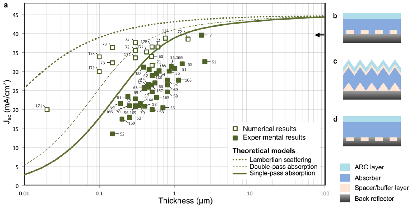
Figure 4. State-of-the-art of ultrathin CIGS solar cells. (a) Short-circuit current density ( J_{sc} ) of thin ( > 400 \text{ nm} ) and ultra-thin ( < 400 \text{ nm} ) CIGS solar cells as a function of the absorber thickness 7,51-73,165-173 . Experimental results are indicated with filled squares. J_{sc} values from numerical calculations are indicated with open squares. All reported values are compared to the reference models defined in Box 1 (curves). The J_{sc} value of the best-efficiency CIGS solar cell is indicated by an arrow. (b-d) Sketches of notable advanced light-trapping schemes used in state-of-the-art ultrathin CIGS cells: (b) back dielectric nanostructure arrays 64 , (c) deposition on textured substrates 72 and (d) nanostructured back mirror 73 .
