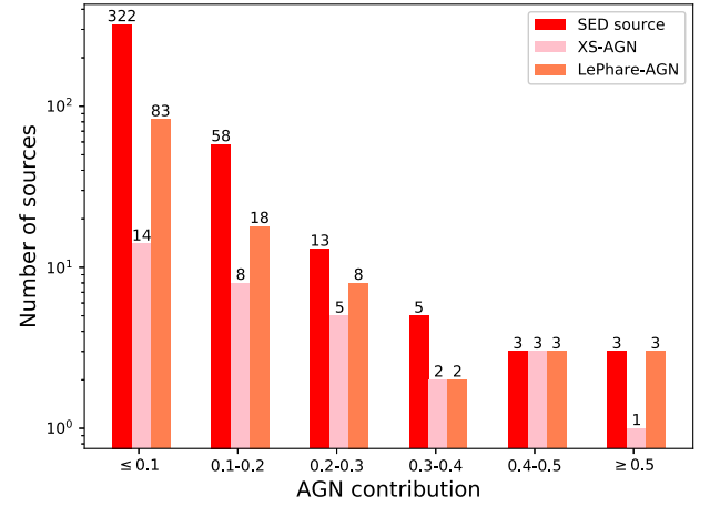
Figure 7. Distribution of the sources at different AGN contribution bin from the spec-z sample. Along x-axis, there are six bins of different AGN contribution. The red bars are the number of the sources in different AGN contribution bins with our method. The pink bars are the number of XS-AGNs in different AGN contribution bins. The orange bars are the number of LePhare-AGNs in different AGN contribution bins.
