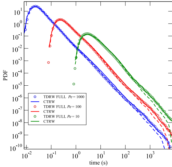
Fig. 12. Comparison of PDFs of the total t_t \tilde{\psi}_t computed using the TDRW for the FULL model with those resulting from the CTRW using as input the mobile time PDFs \tilde{\psi}_m computed using the TDRW model for Pe = 10, 100 and 1000 for the case where \kappa(\mathbf{x}) = \phi(\mathbf{x})^{1-m} with m = 2.5 and \zeta = 0.1 . The dashed lines display the results of the CTRW using constant trapping rate \gamma = 1.51 .
