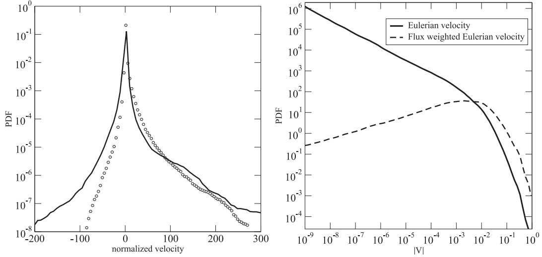
Fig. 2. Left: normalized fluid Eulerian velocity PDF in the direction of the main flow v_z/\bar{v}_z (circles) and in one of the direction perpendicular to the main flow v_x/\bar{v}_z (solid line). Right: Eulerian velocity norm |V| PDF (plain line) and flux weighted Eulerian velocity norm PDF (dashed line).
