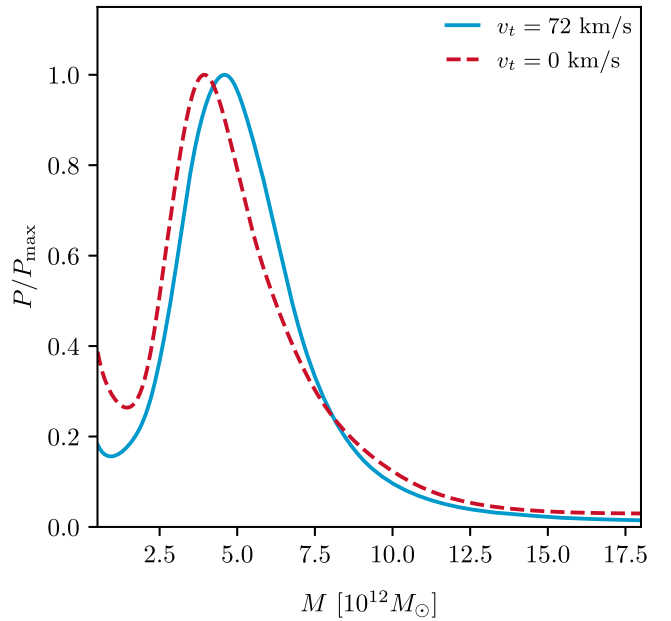
FIG. 9. The posterior on M_{MW+M31} for different values of the tangential velocity: v_t = 72 \text{ km s}^{-1} as used in this work (solid blue), and a purely radial motion v_t = 0 (dashed red).
