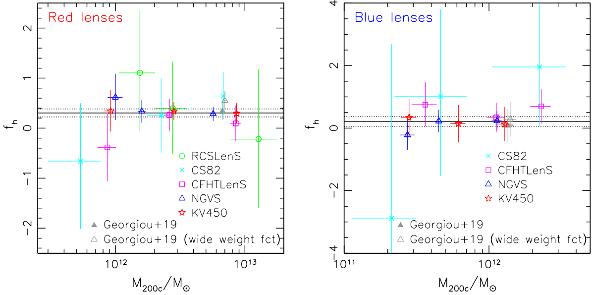
Fig. 2. Constraints on f_h and M_{200c} from the different surveys for red ( left ) and blue ( right ) lenses. For each survey, the different data points correspond to the different stellar mass bins. The horizontal solid and dotted lines mark the best-fit joint f_h constraints and the \pm 1\sigma limits, respectively. For comparison we also show results from the KiDS-1000 analysis of central galaxies from Georgiou et al. (2019b) , including their default constraints and their results achieved using a wider weight function for the shape measurements (shown with an offset in mass for clarity).
