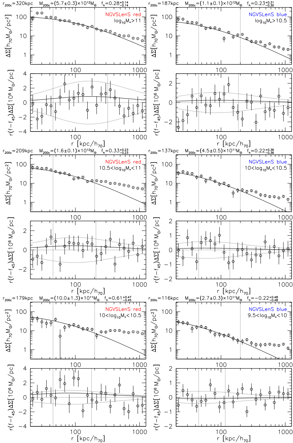
Fig. 1. Measured isotropic (top sub-panel in each panel) and anisotropic (bottom sub-panel in each panel, note the varying y-axis scale) shear signal around red ( left ) and blue ( right ) lenses in the NGVSLenS fields. From top to bottom: decreasing stellar mass bins as indicated. For better readability the anisotropic signal has been scaled by r . The best-fitting NFW shear profile constrained within 45 \text{ kpc}/h_{70} < r < 200 \text{ kpc}/h_{70} is shown by the curve for the isotropic signal. For (f - f_{45})\Delta\Sigma the curves show models computed from the best-fit isotropic model and the best-fit f_h for the solid curve, and f_h \in \{+1, 0, -1\} for the dotted curves, respectively. The best-fit f_h has been constrained from (f - f_{45})\Delta\Sigma and \Delta\Sigma within 45 \text{ kpc}/h_{70} < r < r_{200c} (range indicated by vertical lines), where r_{200c} has been estimated from the isotropic signal. The corresponding figures for the other surveys are shown in Appendix C.
