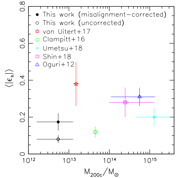
Fig. 4. Comparison of constraints on \langle |\epsilon_h| \rangle for red galaxies, galaxy groups, and galaxy clusters from different studies. For our study we combine the constraints from all red lens samples for our two highest stellar mass bins, showing both the uncorrected estimate (assuming perfect alignment of galaxies and haloes), and the more realistic misalignment-corrected estimate. The latter assumes that the impact of misalignment is correctly described by the comparison of the results from the S15 Millennium Simulation analyses with and without misalignment (see Sect. 5). The horizontal error-bars indicate the approximate lens mass range for our results as well as the studies from Oguri et al. (2012), Shin et al. (2018) and Umetsu et al. (2018). For van Uitert et al. (2017) the data point is shown at their best-fit mean mass, where the error corresponds to the fit uncertainty. Clampitt & Jain (2016) only report an approximate mean mass for their sample. We apply mass conversions in case authors employ other definitions than M_{200c} .
