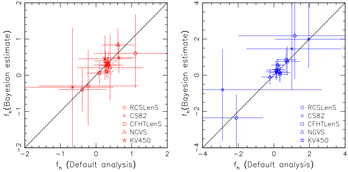
Fig. B.1. Comparison of f_h estimates for the different surveys and lens stellar mass bins from our default analysis scheme (see Sect. 3.4.3) and the Bayesian estimation described in Appendix B. Left and right panels: red and blue lens samples, respectively.
