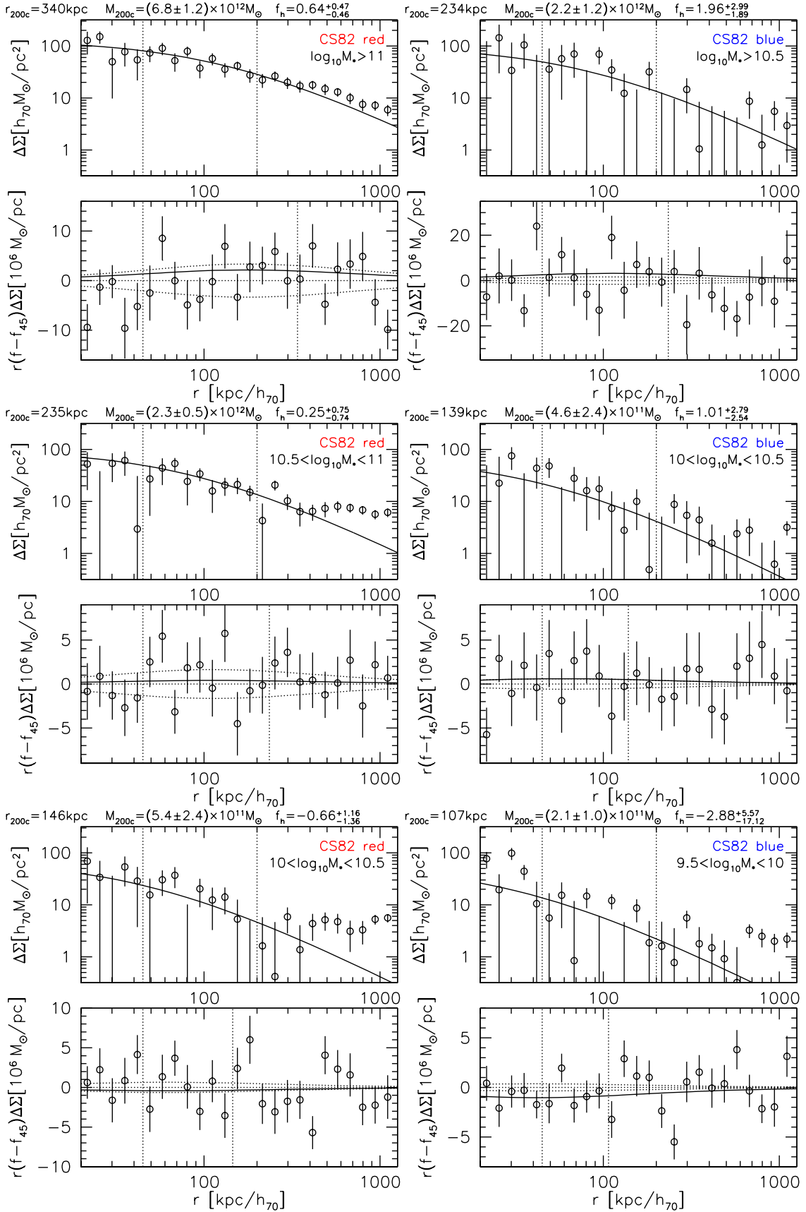
Fig. C.3. As Fig. 1, but computed from the CS2 data.
