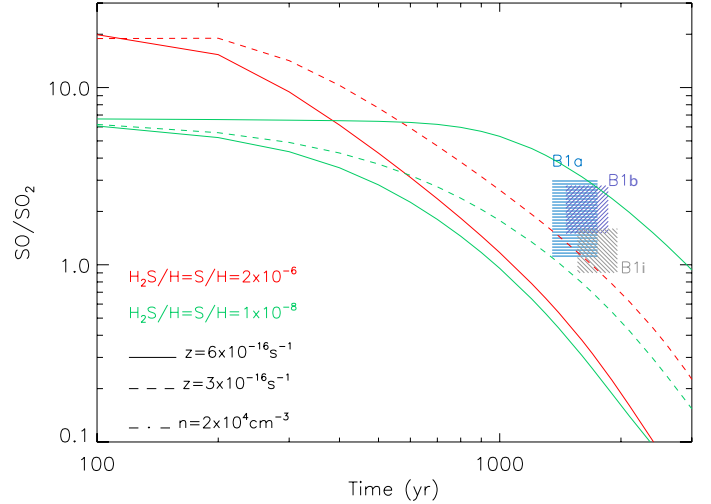
Figure 8. SO/SO 2 abundance ratio predicted by our astrochemical model (see text) as a function of the time for different H 2 S/H and S/H abundances, 2 \times 10^{-6} (red curves) and 1 \times 10^{-8} (green curves). The model predictions are also obtained for two values of the cosmic rays ionization rates, 6 \times 10^{-16} \text{ s}^{-1} (solid curves) and 3 \times 10^{-16} \text{ s}^{-1} (dashed curves), and a smaller H density, 2 \times 10^4 \text{ cm}^{-3} (dotted-dashed curve). The results from the analysis of the observations are reported in the dashed areas toward three positions along the B1 region: B1a, B1b, and B1i, respectively.
