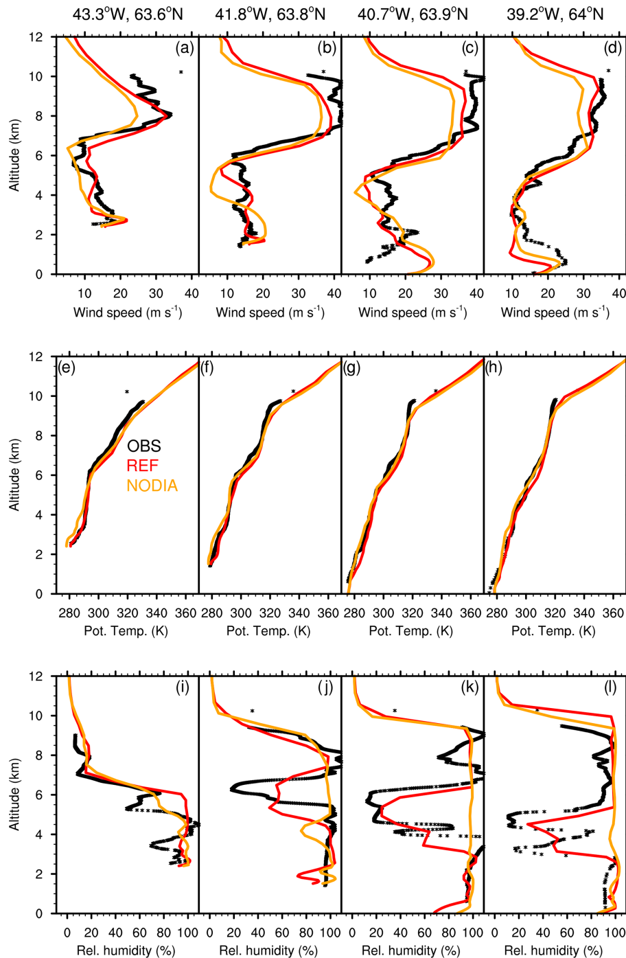
Figure 4. Profiles of (a–d) wind speed, (e–h) potential temperature and (i–l) relative humidity at the following coordinates: (a, e, i) 43.3° W, 63.6° N; (b, f, j) 41.8° W, 63.8° N; (c, g, k) 40.7° W, 63.9° N; and (d, h, l) 39.2° W, 64° N. The dropsondes were launched at 10:26, 10:32, 10:36 and 10:41 UTC, respectively. Their location is shown as white stars in Fig. 1a. The measurements by dropsondes are shown with black lines, and the REF and NODIA simulations are shown with red and orange lines, respectively.
