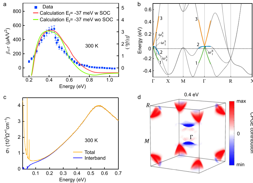
Fig. 3 Room temperature CPGE spectrum, optical conductivity and band structure for CoSi. a Measured second-order CPGE photo-conductivity ( \beta_{xxt} ) as a function of incident photon energy, and ab-initio calculations of the CPGE current with and without spin-orbit coupling at room temperature. b The band structure of CoSi without spin-orbit coupling. We define zero energy at the threefold node at the \Gamma point. The double Weyl node at the R point is at -185 meV. The dashed horizontal line indicates the chemical potential E_f = -37 meV in our sample, moderately lower from that obtained by DFT ( E_f = -20 meV). The band structure of the \mathbf{k} \cdot \mathbf{p} model is shown in green (band 1), blue (band 2), and orange (band 3) obtained by fitting the ab-initio band structure (black) up to quadratic corrections. For the \Gamma-X direction we define \omega_1^x , \omega_2^x , and \omega_3^x as the minimum energy that allows transitions from band 1 to band 2, the maximum energy that allows transition from band 1 to band 2 and the minimum energy that allows transitions from band 2 to band 3, respectively. We define in the same way \omega_1^R in the R direction ( \omega_{2,3}^R fall outside the applicability of the quadratic model). c Total (gold) and interband (blue) optical conductivity of CoSi at 300 K. d Momentum resolved contributions to the CPGE peak at 0.4 eV in the red curve in a .
