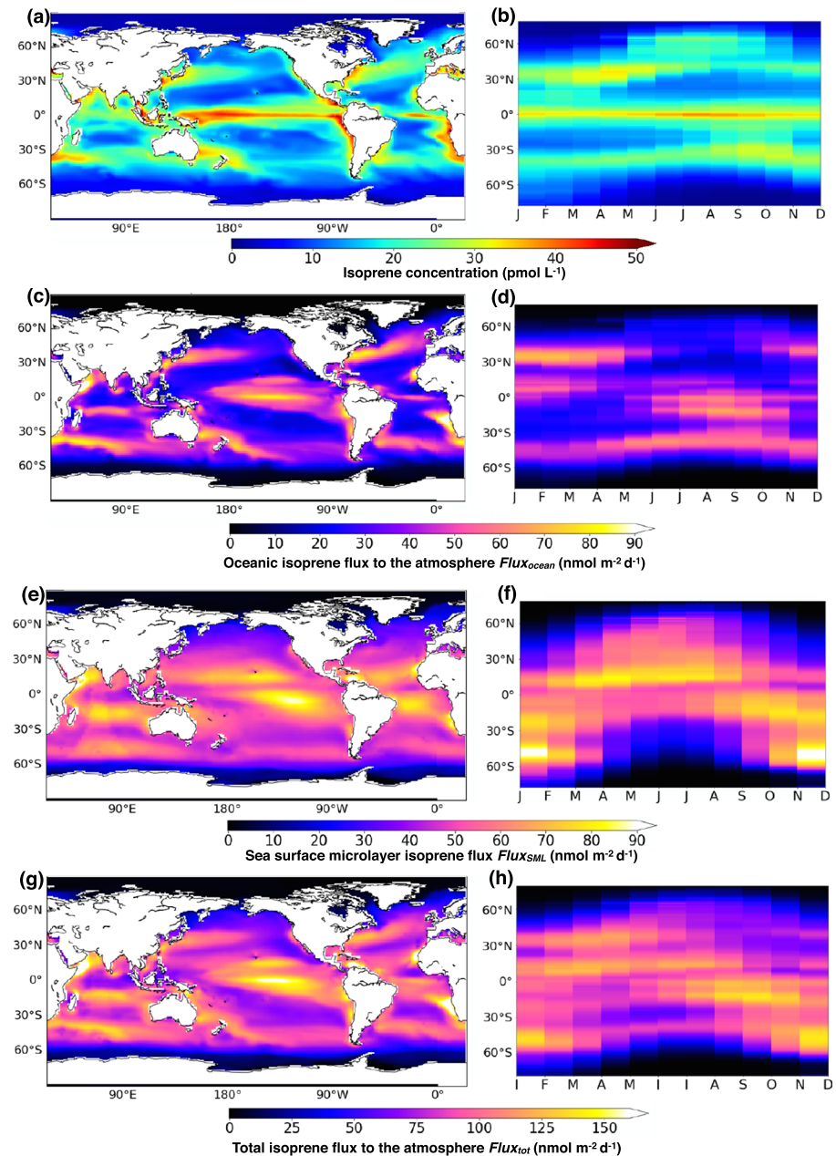
Figure 8. Oceanic isoprene concentration between 0 and 10 m (a and b), oceanic isoprene flux to the atmosphere Flux_{ocean} (c and d), sea surface microlayer flux Flux_{SML} (e and f), and total flux to the atmosphere Flux_{tot} (g and h). (a, c, e, and g) Spatial distribution of the annual mean. (b, d, f, and h) Mean seasonal variation with latitude.
