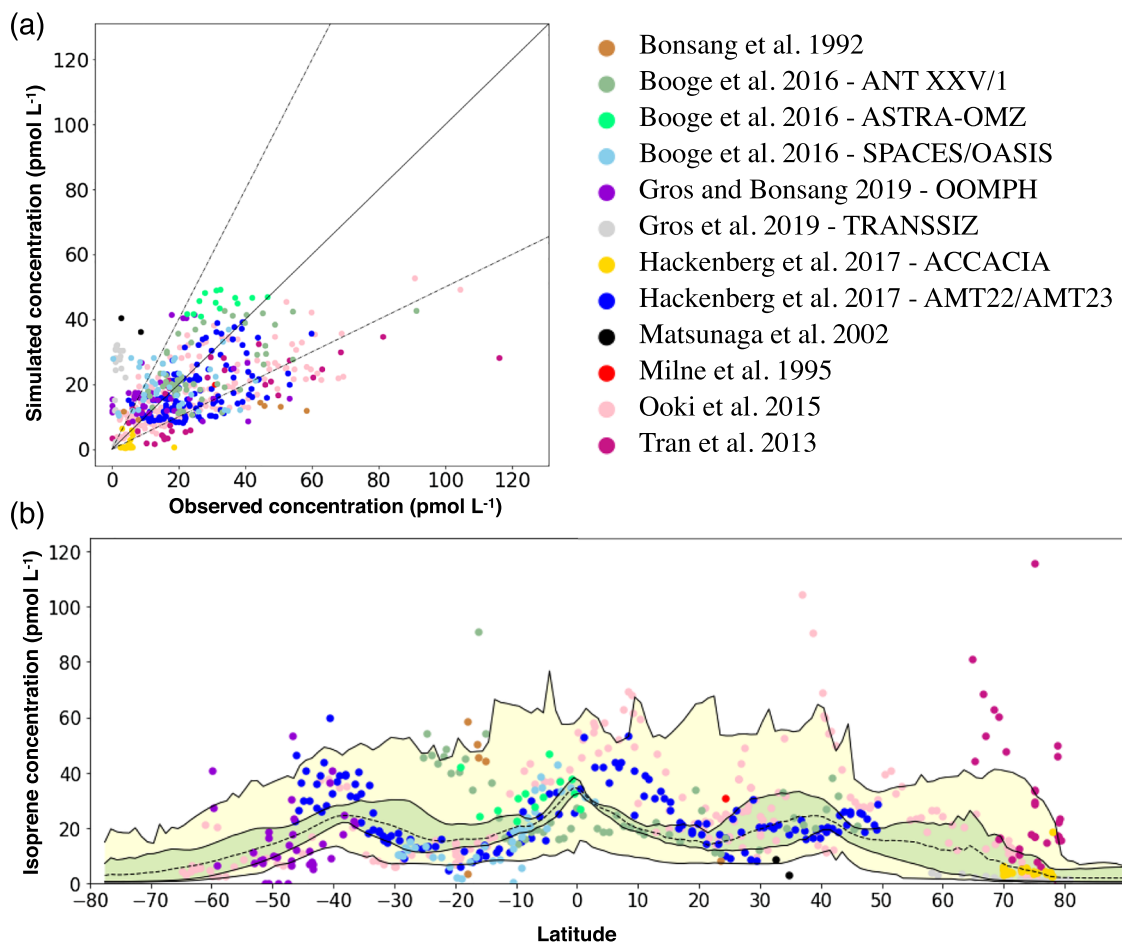
Figure 3. Comparison between simulated and observed isoprene concentrations in the surface ocean for the standard experiment. (a) Comparison using a scatter plot (the solid line represents the 1–1 line and dotted lines the 1–2 and 2–1 lines). (b) Surface concentrations as a function of the latitude (dots: observed concentrations; dotted line: longitudinal and monthly mean simulated isoprene concentration; green area: interval between maximum and minimum longitudinal mean concentrations; yellow area: interval between maximum and minimum concentrations at a given latitude).
