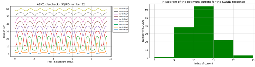
Fig. 6 Left : typical flux response of a QUBIC SQUID for different currents. Right : histogram of the SQUID response as a function of current (expressed in digital unit). (Color figure online.)
