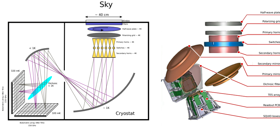
Fig. 1 Left : Schematic of the QUBIC instrument. The window aperture is about 40 cm; the cryostat is about 1.41 m in diameter and 1.51 m in height; Right : 3D rendering of the inner part of the cryostat. TES, Transition Edge Sensor. (Color figure online.)
