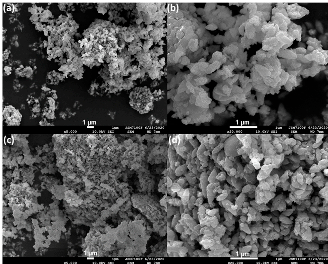
Figure 3. Representative scanning electron microscopic (SEM) images of the samples, (a) Zn4La—5000×, (b) Zn4La—20,000×, (c) Zn4La400—5000× and (d) Zn4La400—20,000×.
