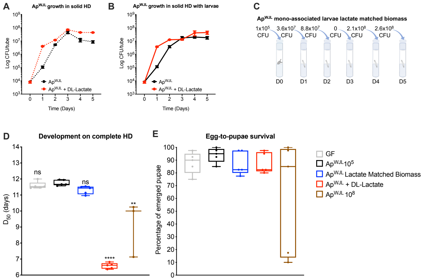
Figure S3. Related to Figure 3: (A-B) Load of Ap^{WJL} in solid HD supplemented (red) or not (black) with DL-lactate at a final concentration of 0.6 g/L with (B) and without (A) larvae, from day 0 to 5 days after inoculation. (C) Graphical representation of the daily Ap^{WJL} biomass supplementation to Ap^{WJL} mono-associated larvae in order to match the biomass reached upon DL-lactate supplementation, according with Fig. S3B. (D) Developmental timing of Germ Free (GF, light grey) larvae or GF larvae inoculated with 10^5 CFU of Ap^{WJL} (black) or Ap^{WJL} mono-associated larvae supplemented daily with live Ap^{WJL} biomass (blue) or DL-lactate (red) and GF larvae inoculated with 10^8 CFU of Ap^{WJL} (brown). (E) Percentage of the emerged pupae from the developmental timing experiment of Fig. S3D. Symbols represent the means \pm SEM of three biological replicates except for panel (A-B). Boxplots show minimum, maximum and median. Points represent biological replicates. We performed Kruskal-Wallis test followed by
