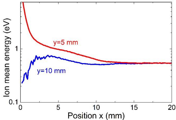
Figure 13: Axial profiles of the ion mean kinetic energy at two y locations; in the center of a cusp, y=5 mm and at a mid-position between two cusps, y=10 mm. Same conditions as Figure 5: B_0=400 G, Argon, 0.1 mtorr, T_e=2 eV, T_i=0.5 eV.
