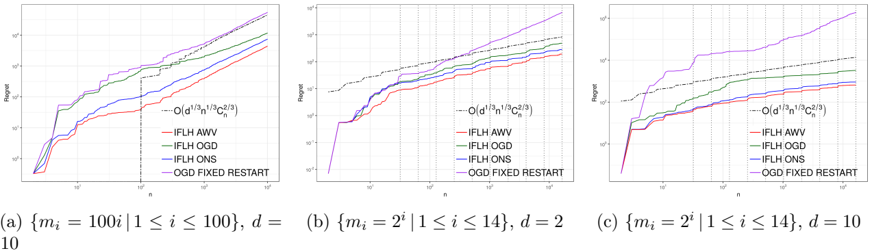
Figure 4: Performances of online linear regression IFLH algorithms and OGD with fixed restart on the time series generated with the Hard Shifts.
