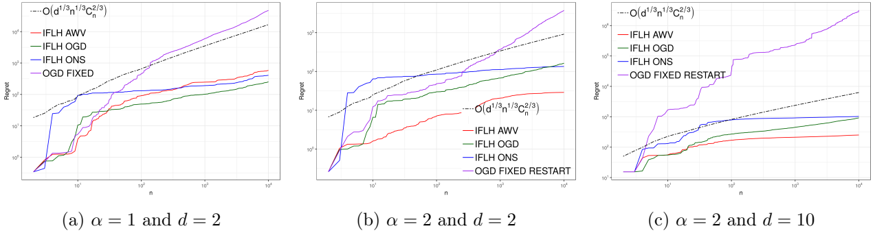
Figure 3: Performances of online linear regression IFLH algorithms and OGD with fixed restart on the time series generated with the Soft Shifts for various dimension d and parameter \alpha
