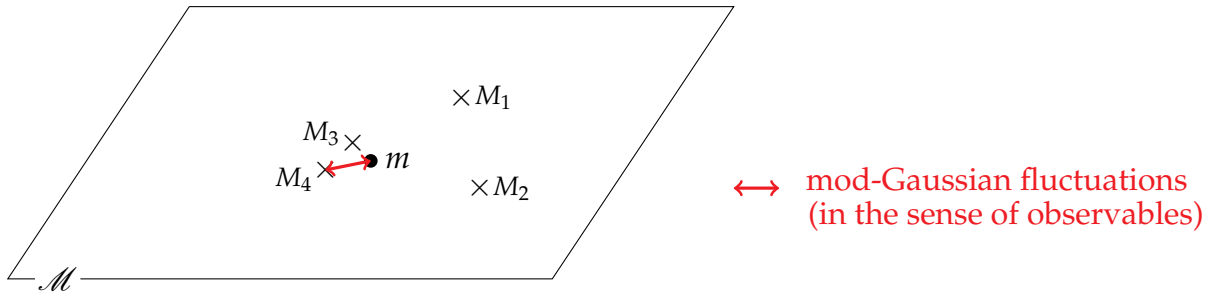
FIGURE 13. Mod-Gaussian moduli spaces as fields of fluctuations.
