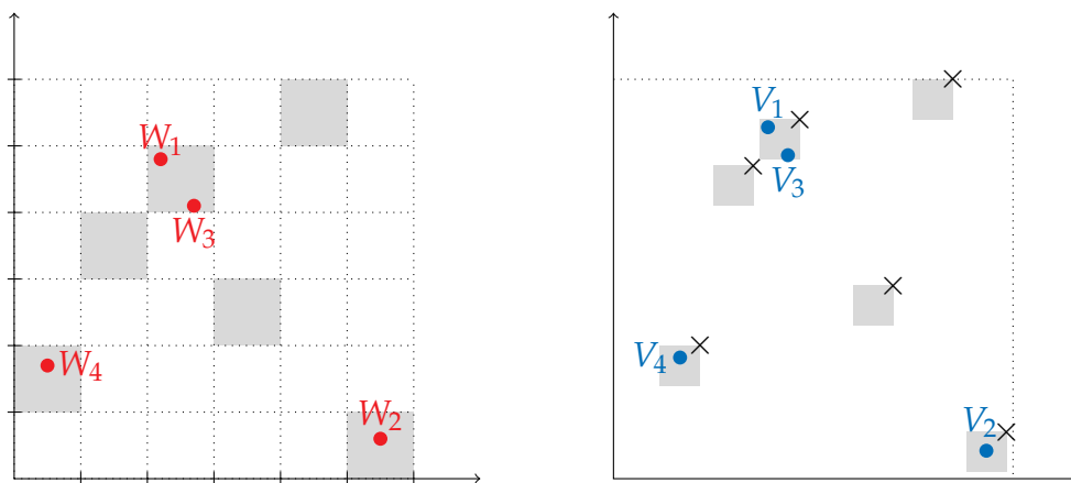
FIGURE 11. The random points W_1, \dots, W_k and V_1, \dots, V_k have the same configuration.
