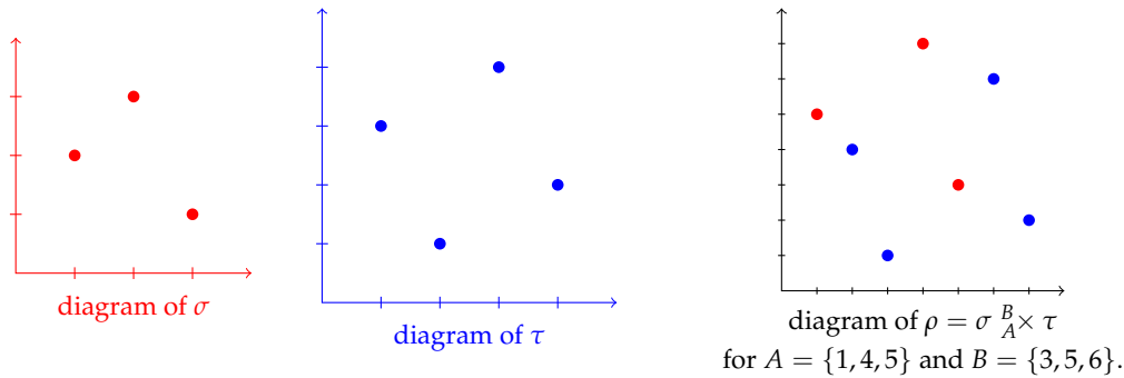
FIGURE 9. Example of (A, B) -shuffle of permutations.
