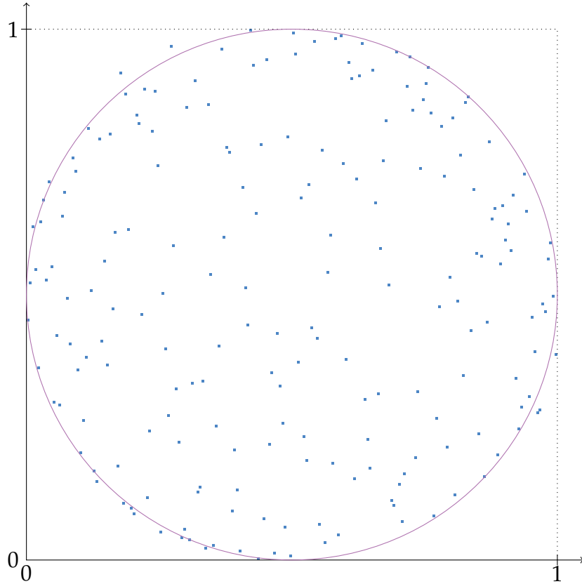
FIGURE 7. Diagram of a random permutation with size n = 200 associated with the permuton with density 1_{d((x,y),(\frac{1}{2},\frac{1}{2})) \leq \frac{1}{2}} \frac{2}{\pi \sqrt{1-4(x-\frac{1}{2})^2-4(y-\frac{1}{2})^2}} dx dy .
