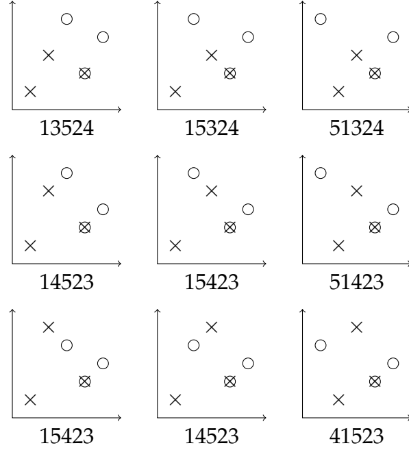
FIGURE 12. The permutations involved in the amalgamated graphical shuffle product of \tau = 312 and \rho = 132 at (a, b) = (2, 3) .
