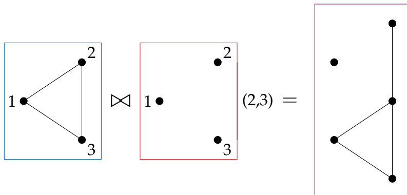
FIGURE 10. The junction (F \bowtie G)(a, b) of two graphs along a pair of points (a \in V_F, b \in V_G) .
