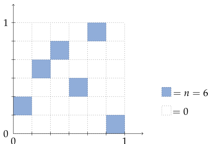
FIGURE 6. The density of the permuton \pi(\sigma) associated with the permutation \sigma = 245361 .
