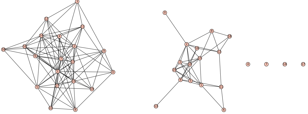
FIGURE 5. Two random graphs of size n = 20 associated with the graph functions g(x, y) = \frac{x+y}{2} and g'(x, y) = xy .
