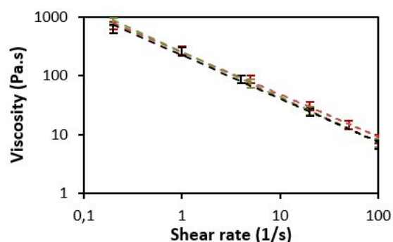
10 Figure 4. Viscosity plots of a pure HEC solution (black), and HKUST-1-based inks formulated 11 with 11 wt% of large crystals (red) and with 16 wt% of nanocrystals (green). MOF/HEC = 4.9 12 (blue) and 6.9 (green); HEC/PVA = 2.1.
