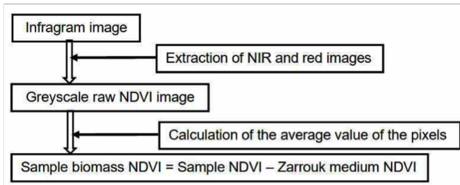
Fig 4. NDVI calculation principle.
