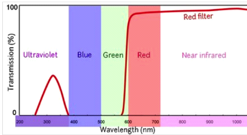
Fig 2. Spectral response of camera redfilter (Source: https://publiclab.org/notes/cfastie/11-24-2015/dual-band-pass-filters )
