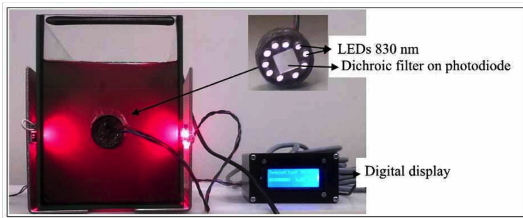
Fig 4. Experimental setup for reflectance signal measurement.
