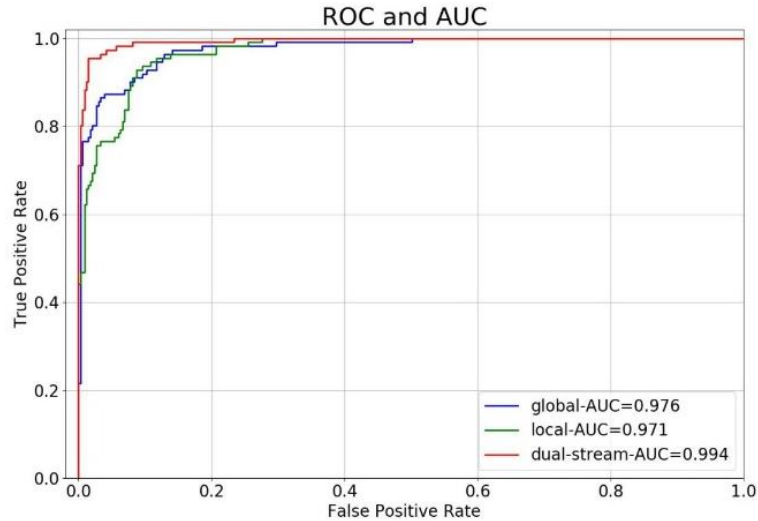
Fig. 8. ROC curves and AUC values of the DSN (Red), the Global Network (Blue) and the Local Network (Green).
