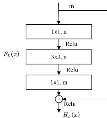
Fig. 7. A building block of residual network.
