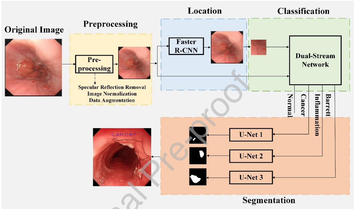
Fig. 3. Overview of the proposed ELNet for esophageal lesion classification and segmentation.
