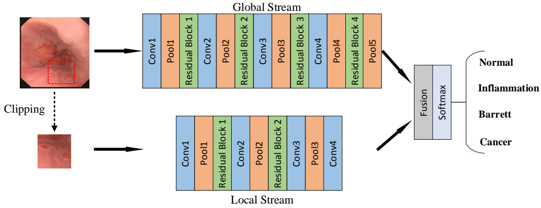
Fig. 6. The structure of the proposed Dual-Stream Network (DSN).
