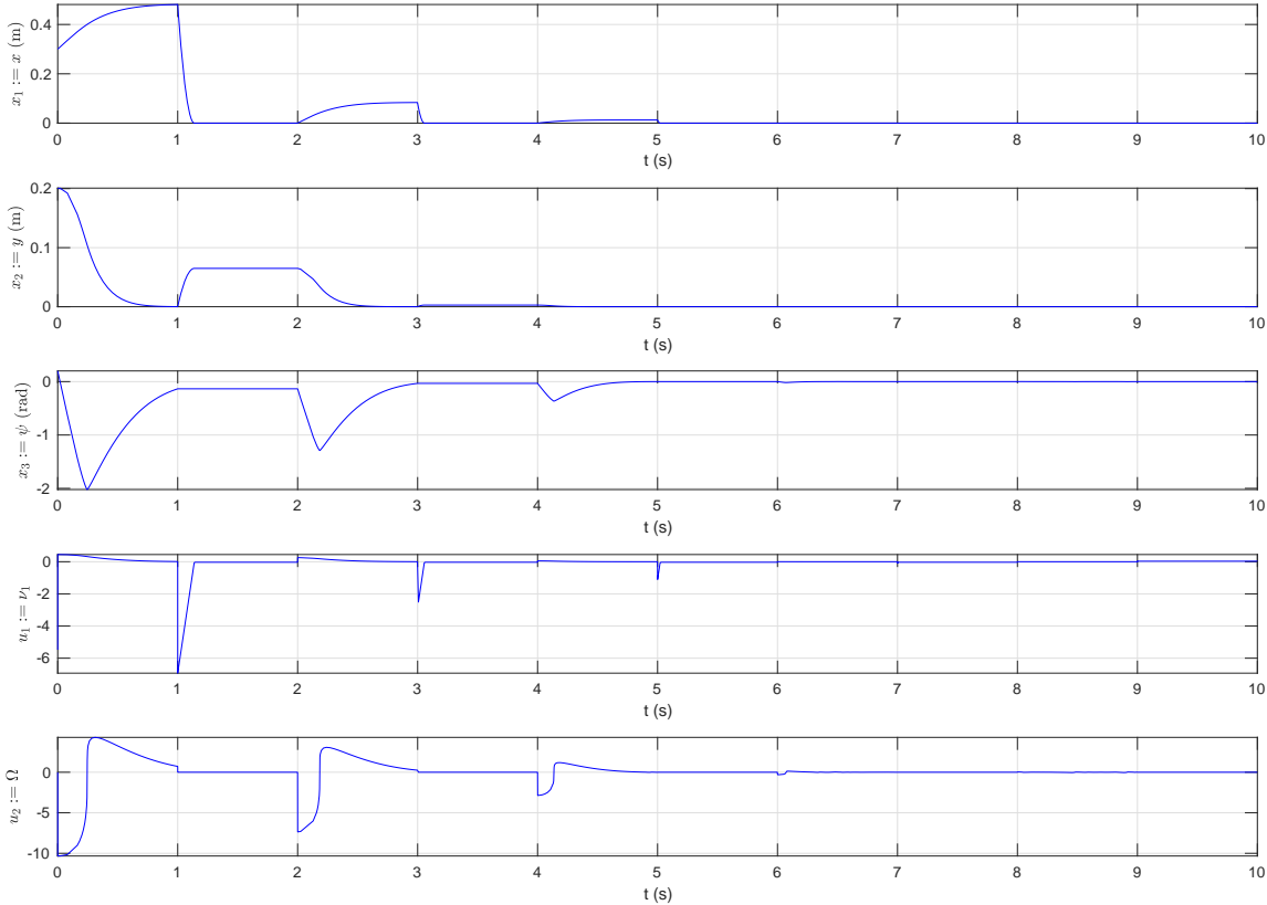
Figure 3: Simulation of (4.2) using control (4.7) with T = 2, \nu = 0.5; \kappa_1 = -0.5, \kappa_2 = -0.1, l = 3, k_1 = 10, k_2 = k_3 = 5 .
