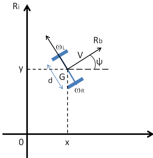
Figure 1: The “unicycle-like” mobile robot
