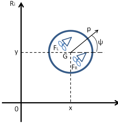
Figure 2: The slider
