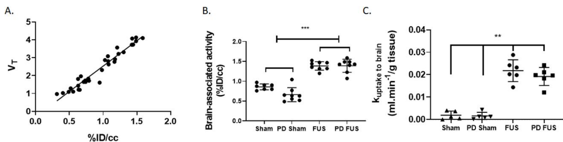
344 Figure 3. Comparison of PET imaging quantification between different groups and 345 pharmacokinetics calculation. A. Correlation between V_T and the concentration of activity (%ID/cc) 346 at 24 h post-injection. B. Concentration of activity in the brain 24 hours after injection in different 347 groups (sham, pharmacologic dose (PD) sham, FUS and pharmacologic dose (PD) FUS). C. Brain 348 uptake transfer ( k_{\text{uptake}} ) of ^{89}\text{Zr} -DFO-CTX in different groups. ** P < 0.01 , n = 8 mice per group.
