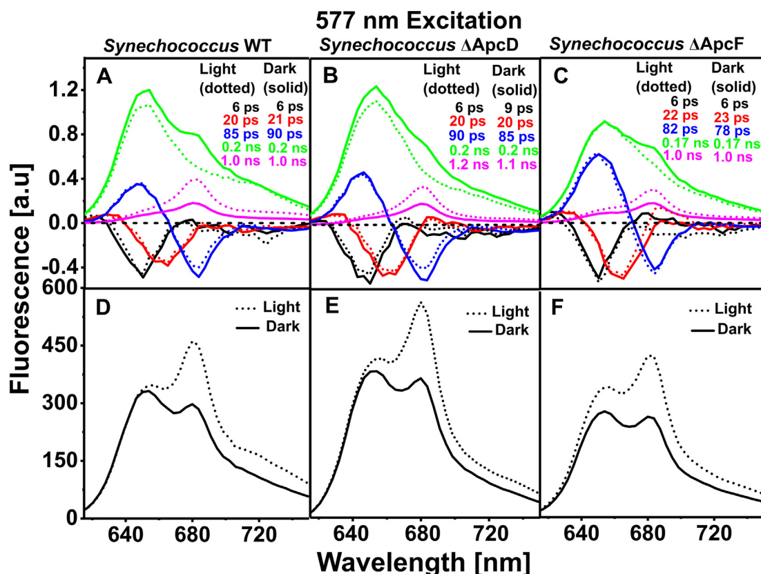
Fig. 4. Decay-associated spectra obtained from global fitting of time-resolved fluorescence results after 577 nm excitation. (A, B, C) five-components DAS of Synechococcus WT, Synechococcus ΔApcD and Synechococcus ΔApcF, in state I (dotted lines) and state II (solid lines). DAS-associated lifetimes are presented in the insets with corresponding colours. In A and C the slowest lifetime is fixed to 1.0 ns. (D, E, F) reconstructed steady-state spectra for Synechococcus WT, Synechococcus ΔApcD and Synechococcus ΔApcF, respectively, in state I (dotted line) and state II (solid line). All spectra are scaled as described in Materials and Methods.
