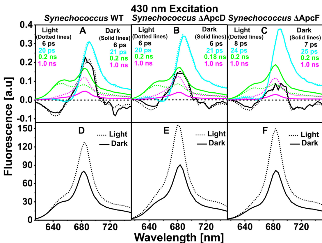
Fig. 5. Decay-associated spectra (DAS) obtained from global fitting of time-resolved fluorescence results upon 430 nm excitation. (A, B, C) four-components DAS of Synechococcus WT, Synechococcus \Delta ApcD and Synechococcus \Delta ApcF, respectively in state I (dotted lines) and state II (solid lines). The slowest lifetime in each case was fixed to 1.0 ns. The \sim 20 ps DAS in each case is multiplied with 0.5 to make the two slowest DAS better visible. DAS-associated lifetimes are shown in the legend with corresponding colours. (D, E, F) reconstructed steady-state spectra for Synechococcus WT, Synechococcus \Delta ApcD and Synechococcus \Delta ApcF, respectively in state I (dotted line) and state II (solid line). All spectra are scaled as described in Materials and Methods.
