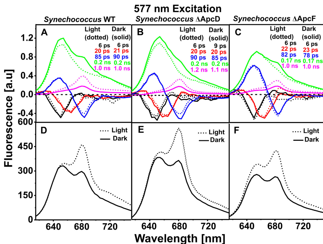
Fig. 4. Decay-associated spectra obtained from global fitting of time-resolved fluorescence results after 577 nm excitation. (A, B, C) five-components DAS of Synechococcus WT, Synechococcus \Delta ApcD and Synechococcus \Delta ApcF, in state I (dotted lines) and state II (solid lines). DAS-associated lifetimes are presented in the insets with corresponding colours. In A and C the slowest lifetime is fixed to 1.0 ns. (D, E, F) reconstructed steady-state spectra for Synechococcus WT, Synechococcus \Delta ApcD and Synechococcus \Delta ApcF, respectively, in state I (dotted line) and state II (solid line). All spectra are scaled as described in Materials and Methods.
