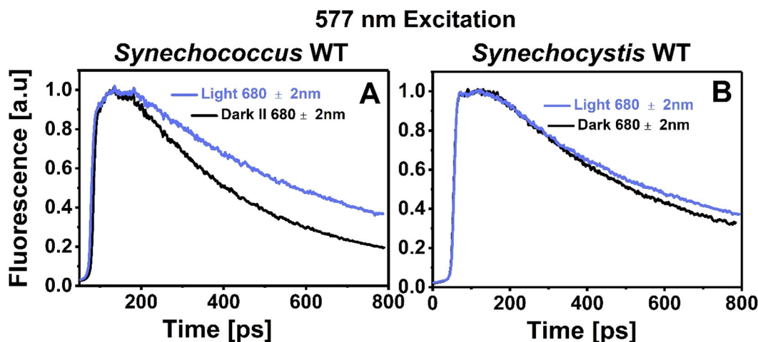
Fig. 3. Normalized decay traces at 680 nm (PBS terminal emitter ( APC_{680} ) and PSII) for dark-adapted (black lines) and light-adapted cells (blue lines) of (A) Synechococcus and (B) Synechocystis . Excitation wavelength was 577 nm and measurements were done at room temperature.
