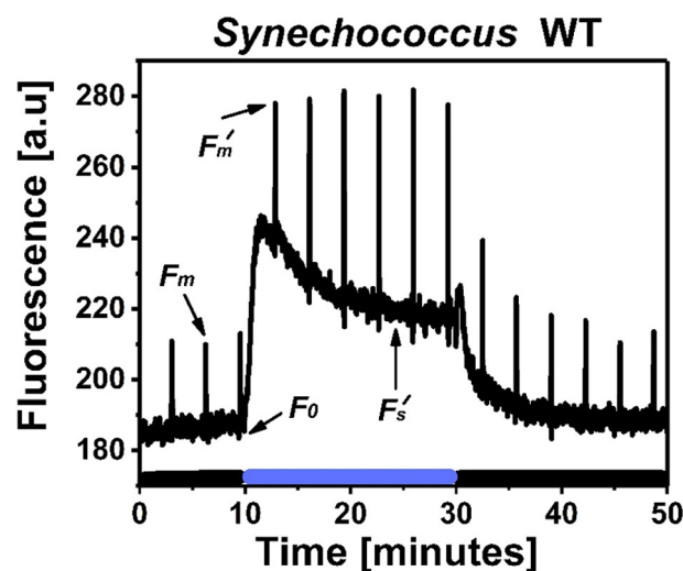
Fig. 1. Time traces of variable fluorescence in wild-type Synechococcus 7942 measured with the pulse-amplitude modulated fluorescence technique. The fluorescence detection window was > 700 \text{ nm} . Black and blue thick solid lines along the time-axis represent the time periods of cells in darkness and blue light respectively. Blue light with central wavelength 452 \text{ nm} and \sim 40 \mu\text{mol photons m}^{-2} \text{ s}^{-1} was used to bring the cells to state I. Blue-light-adapted cells were subsequently put in darkness to bring the cells to state II. F_0 , F_m represent minimum and maximum fluorescence, respectively, for dark-adapted cells. F_s' and F_m' are steady-state and maximum fluorescence, respectively, for cells in blue light.
