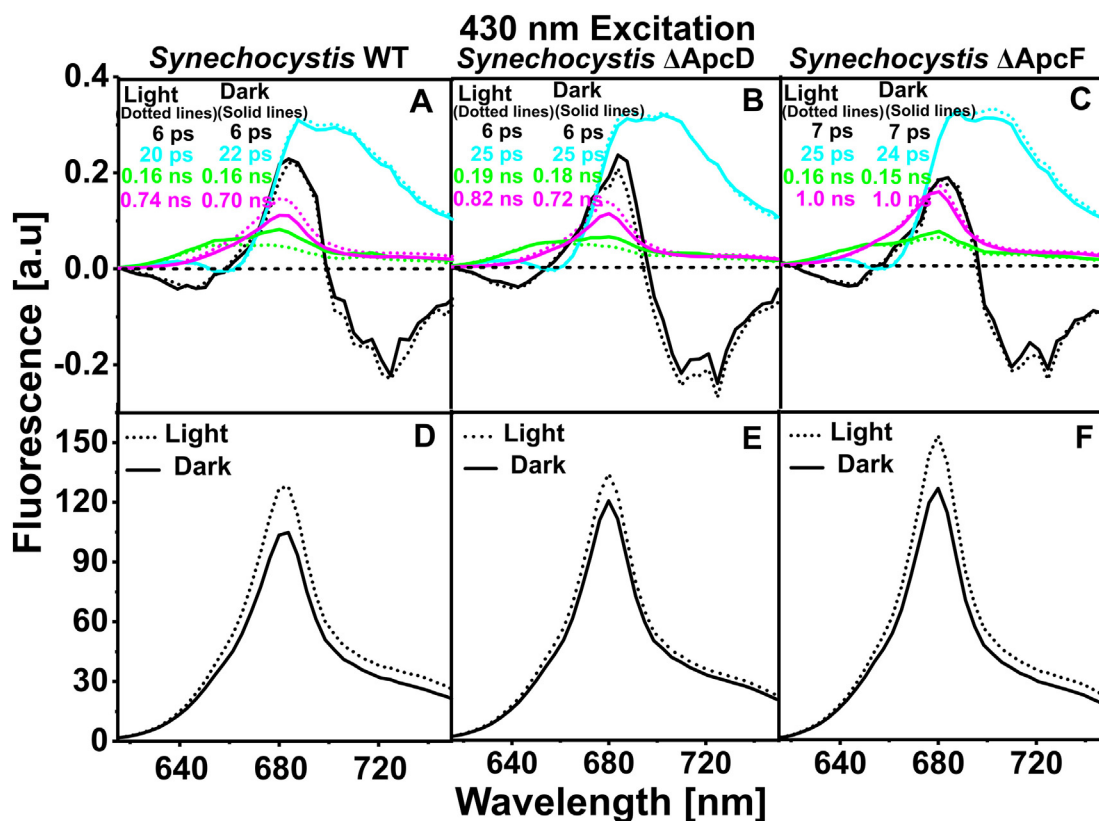
Fig. 7. (A, B, C) four-components DAS of Synechocystis WT, Synechocystis \Delta ApcD and Synechocystis \Delta ApcF, respectively in state I (dotted lines) and state II (solid lines). The 20 ps DAS in each case is multiplied by 0.5 to make the two slowest DAS better visible. DAS-associated lifetimes are presented at the top with corresponding colours. In Figure C the lifetime of the slowest component was fixed to 1.0 ns. (D, E, F) reconstructed steady-state spectra for Synechococcus WT, Synechococcus \Delta ApcD and Synechococcus \Delta ApcF, respectively in state I (dotted lines) and state II (solid lines).
