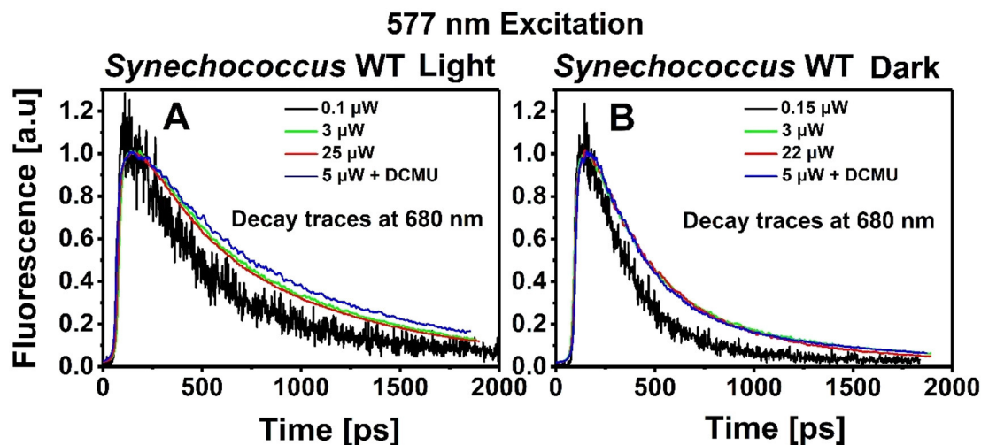
Fig. 2. Fluorescence decay traces of Synechococcus cells at 680 nm obtained with various laser powers after 577 nm excitation (left) light-adapted cells (state I) and (right) dark-adapted cells (state II). Black, green and red traces correspond to cells without DCMU and the blue trace to DCMU-treated cells. All traces were normalized to each other at their maximum emission. Measurements were performed at room temperature.
