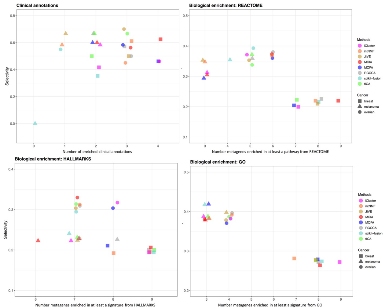
Figure 4. Identification of factors associated with clinical annotations, and metagenes associated with biological annotations in Ovarian, Breast and Melanoma samples, by the jDR methods. For clinical annotations, the plot represents, for each method, the number of clinical annotations enriched in at least one factor together with the selectivity of the associations between the factors and the clinical annotations (Method). For the three annotation sources (MsigDB Hallmarks, REACTOME and Gene Ontology), the number of metagenes identified by the different jDR methods enriched in at least a biological annotation are plotted against the selectivity of the associations between the metagene and the annotation. See Supplementary Figure 2 for the results corresponding to the other seven cancer types.
