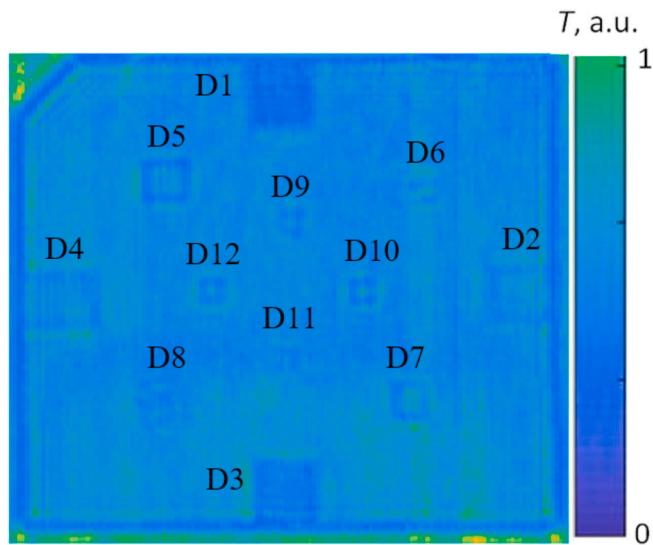
Fig. 12. Terahertz line-scanning results.
