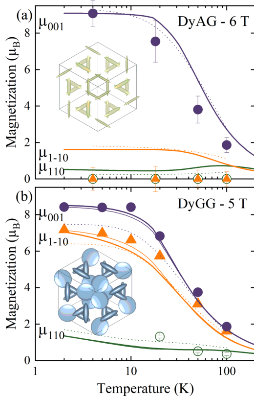
FIG. 4. Magnetization components \mu_{(110)} , \mu_{(\bar{1}\bar{1}0)} and \mu_{(001)} versus temperature for DyAG (a) in 6 T, and for DyGG (b) in 5 T. The insets show magnetic ellipsoids at 5 K. In both panels, dotted lines show susceptibility calculations using the point charge model, and solid lines represent calculations using the CEF model (CEF1 and CEF2 models for DyGG are differentiated by thin and thick lines, respectively). All calculations are based on the parameters given in Table I.
