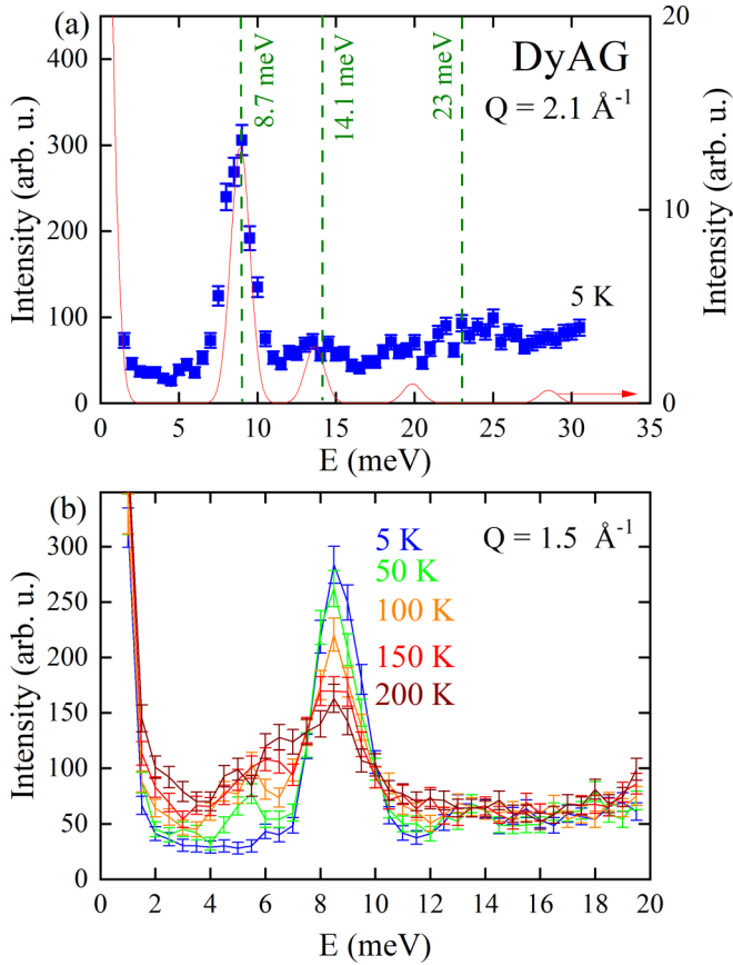
FIG. 5. (a) Constant Q = 2.1 \text{ \AA}^{-1} cut of the S(Q, \omega) of DyAG at 5 K (blue square symbols). In red is shown the neutron cross section calculated for the CEF parameters of Table I. Green lines show the excitation levels determined by optical spectroscopy in Refs. [21,28]. (b) Corresponding temperature evolution of constant Q = 1.5 \text{ \AA}^{-1} scans.
