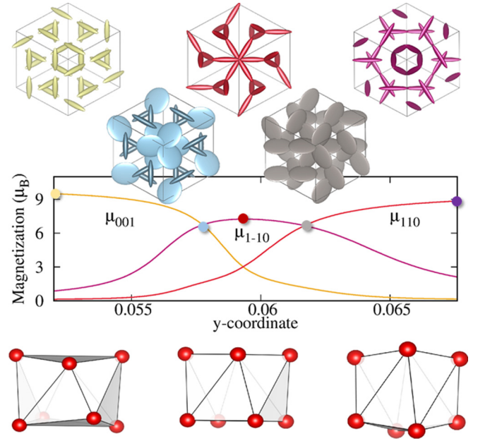
FIG. 7. Evolution of the main ellipsoid axes with the oxygen y position ( 0.03, y, 0.65 ) with effective charge -2e calculated by the point charge model at 5 K in 5 T. The top inserts show the different types of anisotropies obtained for various y coordinates (shown as dots on the graph, of the same color scheme as the inserts). The bottom inserts illustrate the y evolution of the oxygen environment of \text{Dy}^{3+} ion.
