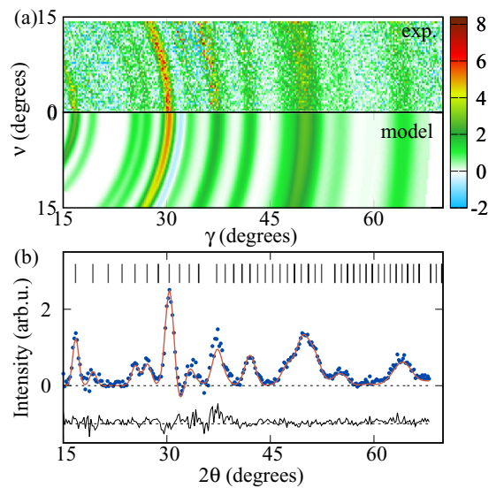
FIG. 3. (a) DyGG flipping difference ( y_+ - y_- ) diffraction pattern collected 5 K and 5 T. (b) Projection on the Bragg angle 2\theta . Notations are the same as for Fig. 2.
