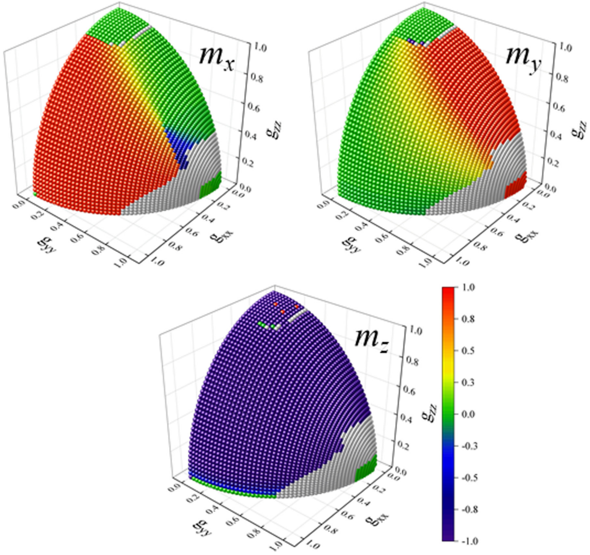
FIG. 16. Variation with g_{xx} , g_{yy} , and g_{zz} of the m_x , m_y , and m_z components written in the local bases of phases AFI and FC (in the latter, m_x , m_y correspond to the 16e site, m_z to the 8b site). Calculations are performed for a pseudospin 1/2 with \mathcal{J} = 1 and x_{\text{dip}} = 100 fixed.
